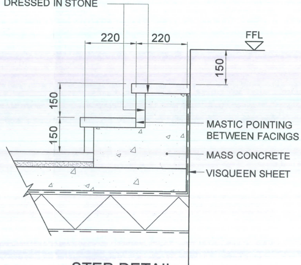
STEP DETAIL (SCALE 1:10)
