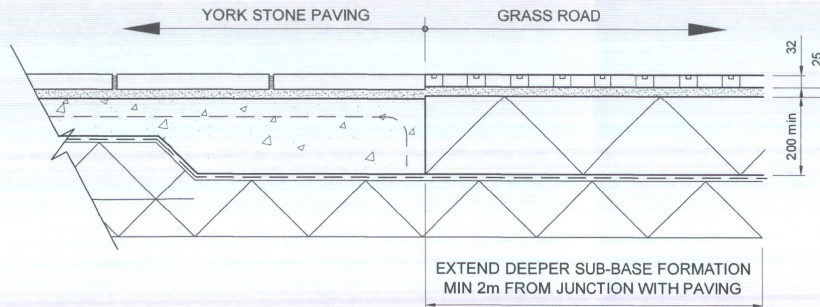
JUNCTION GRASS ROAD / YORK STONE PAVING (SCALE 1:10)
