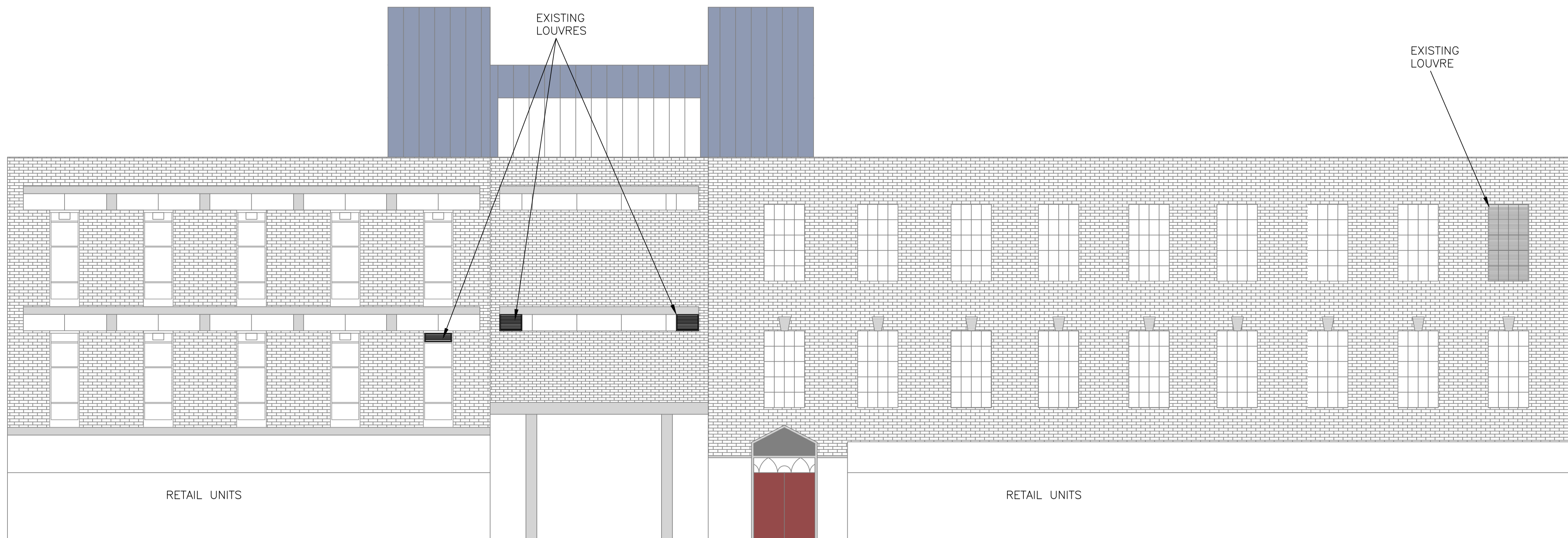
EXISTING EAST ELEVATION (1:100)
