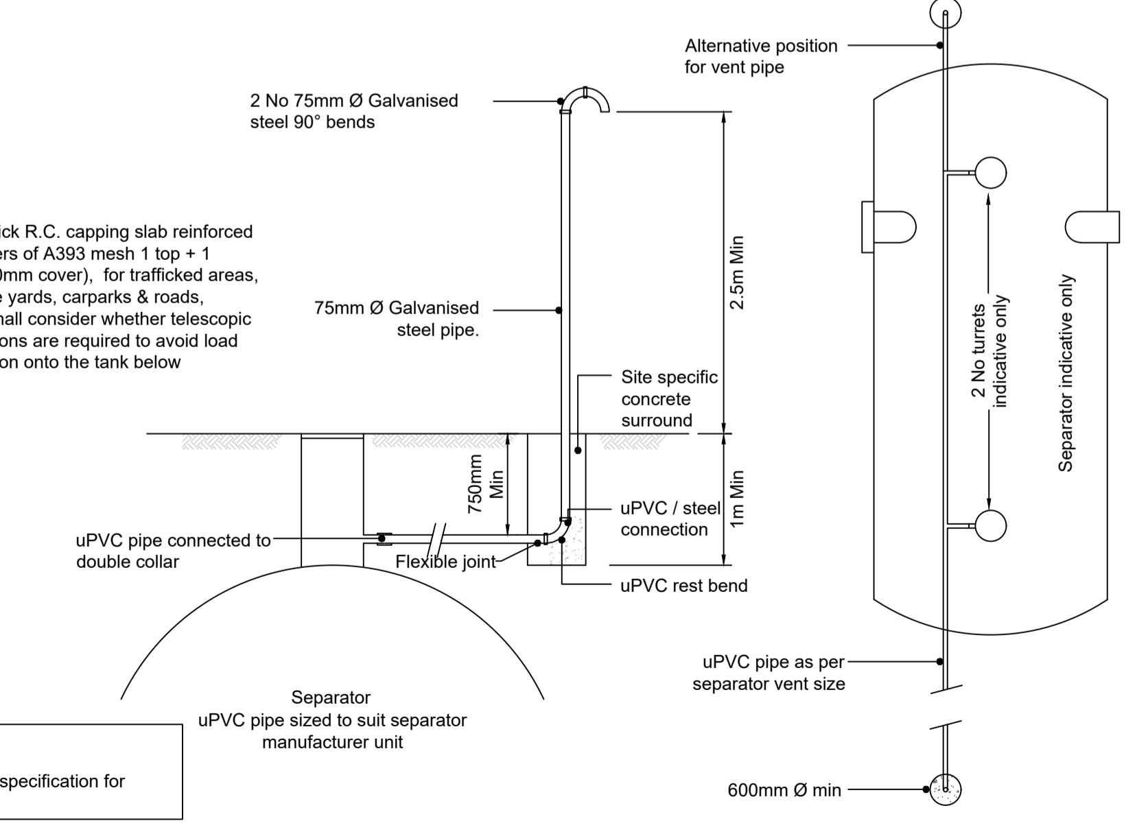
TYPICAL OIL SEPARATOR VENT PIPE DETAIL
