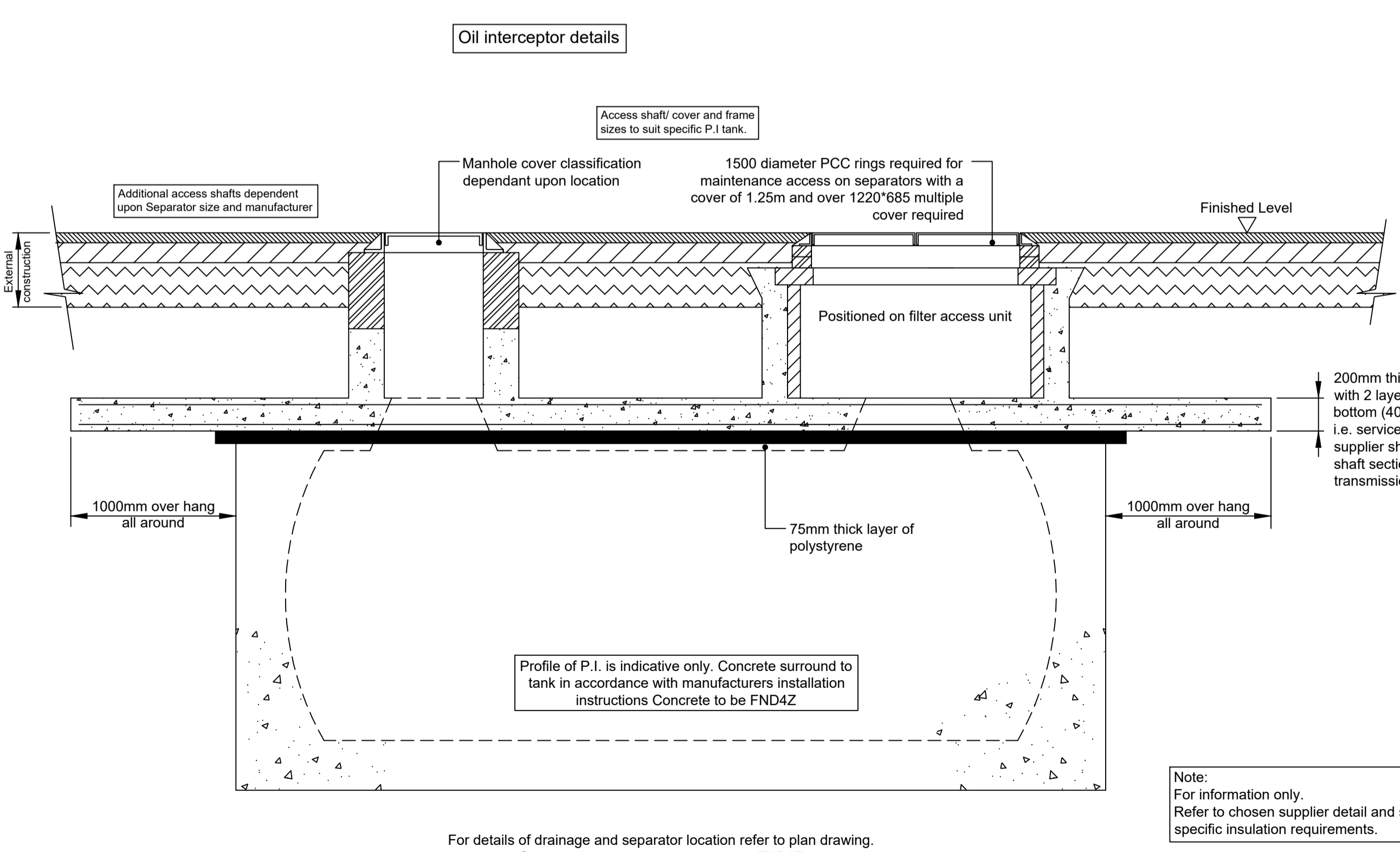
TYPICAL SECTION THROUGH OIL SEPARATOR IN TRAFFICKED AREA
