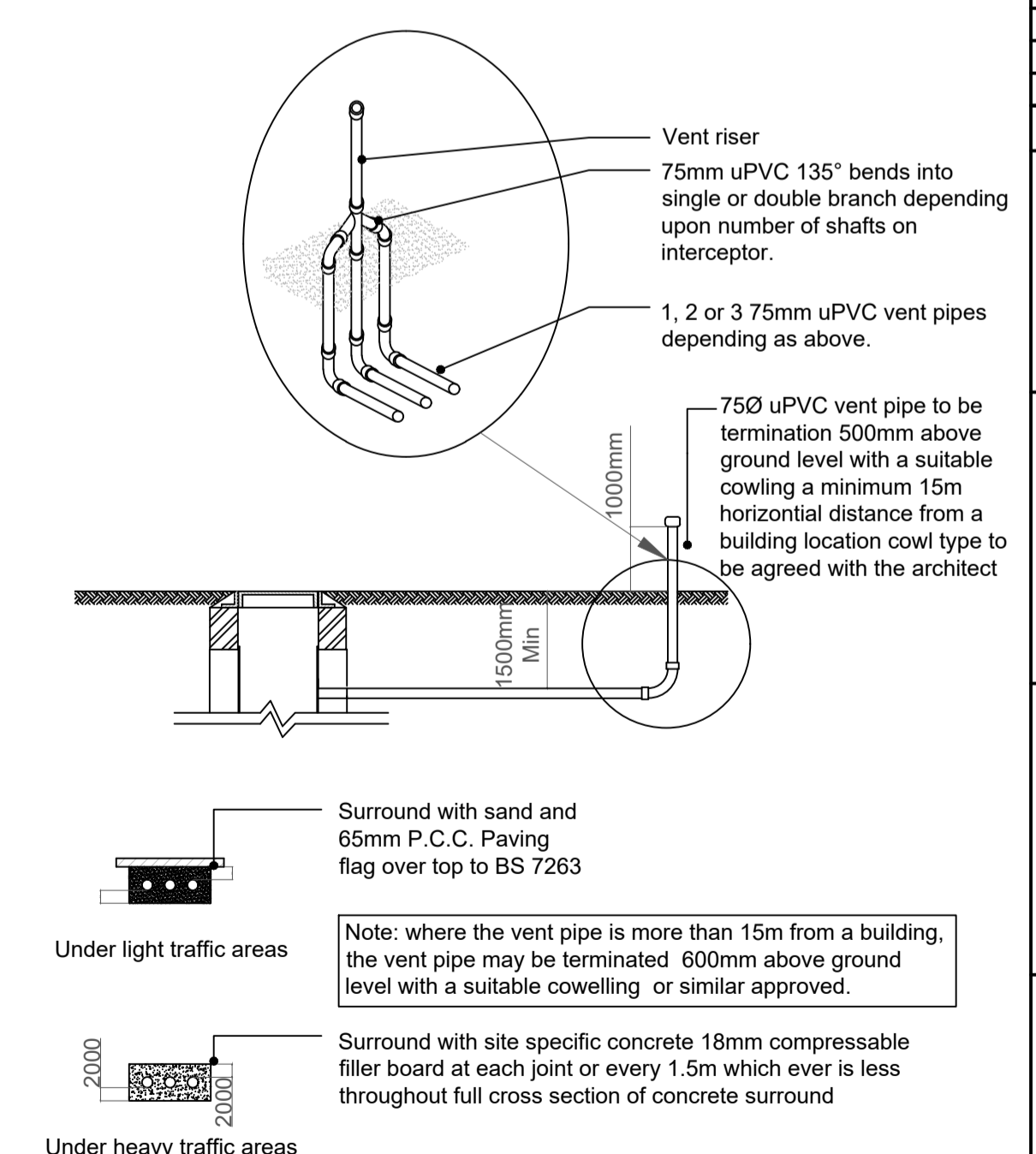
DETAILS OF SURROUNDS TO VENT PIPES
