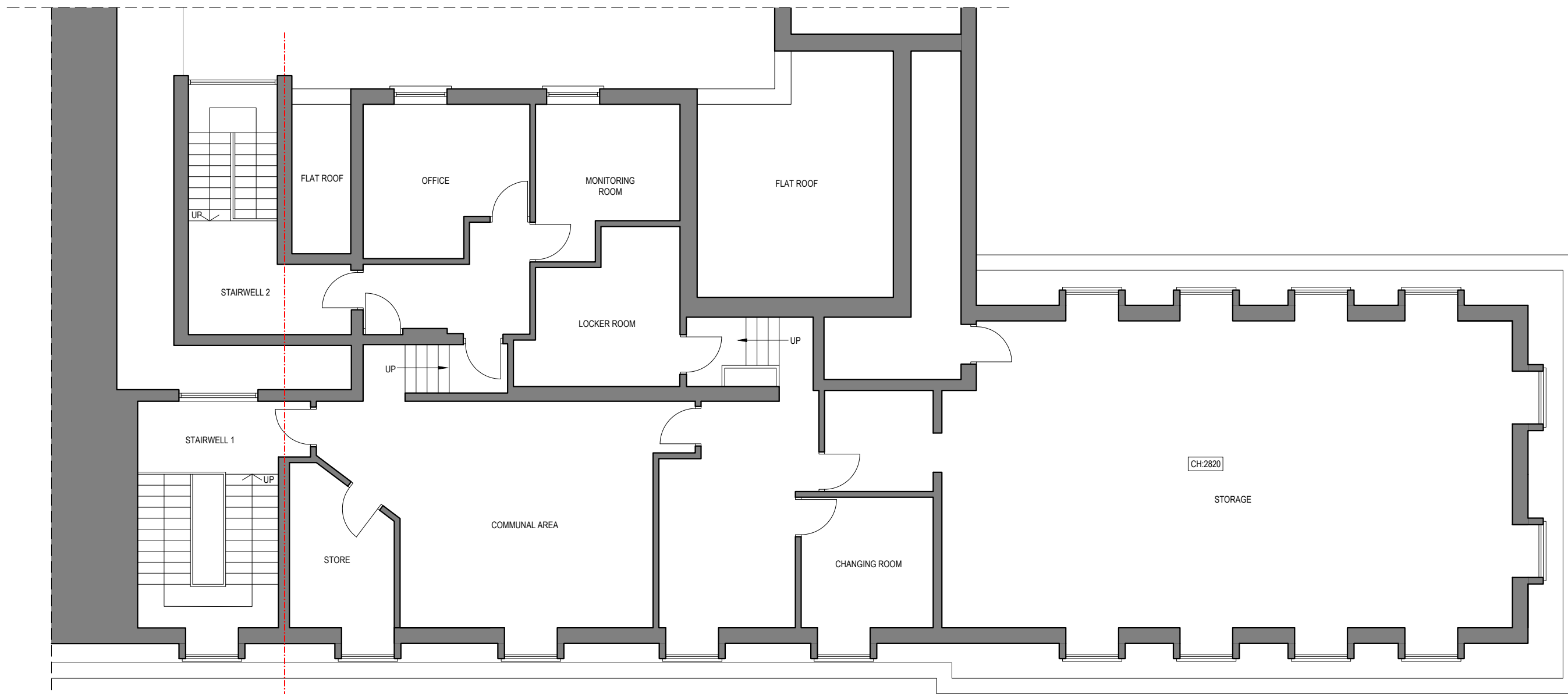
PROPOSED SECOND FLOOR PLAN scale 1:100
