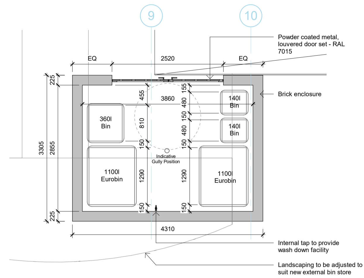
3 External Bin Store 3 - Core G 1 : 50
