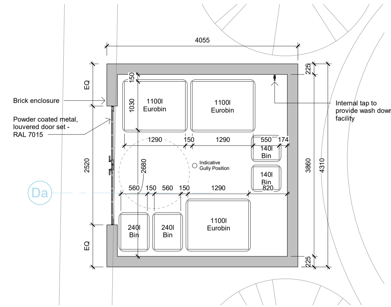
2 External Bin Store 2 - Core F 1 : 50
