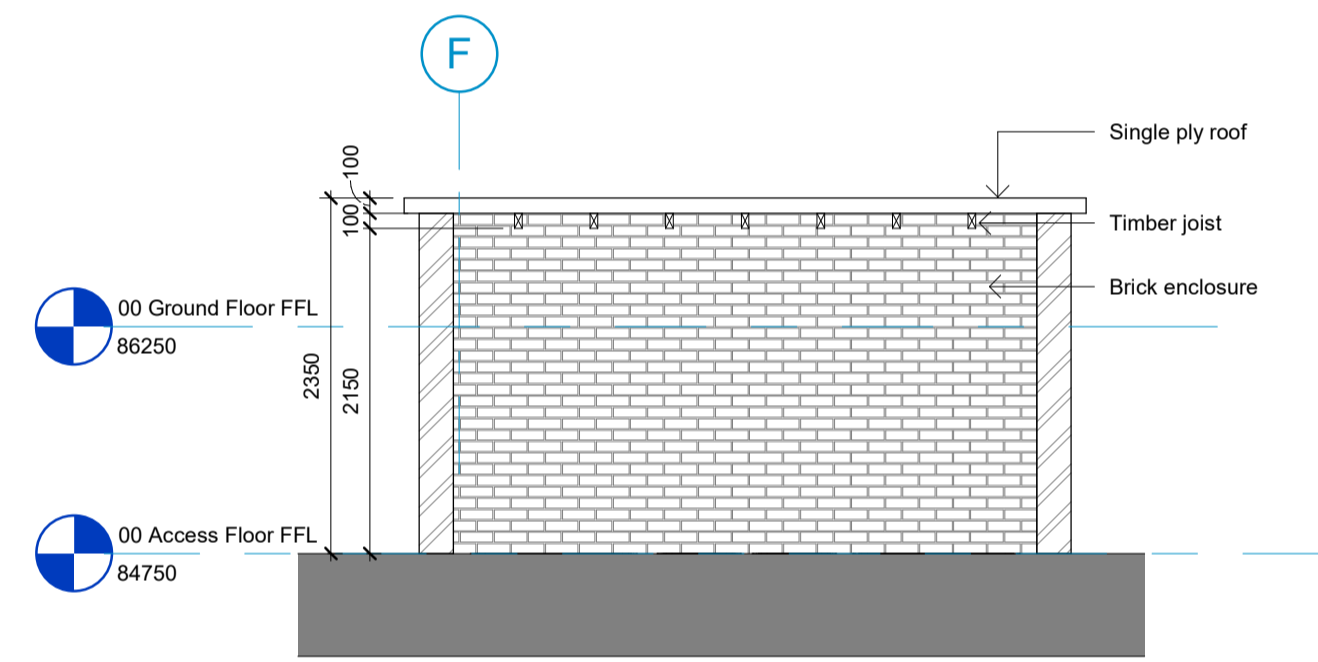
4 Typical External Bin Store Section 1 : 50
