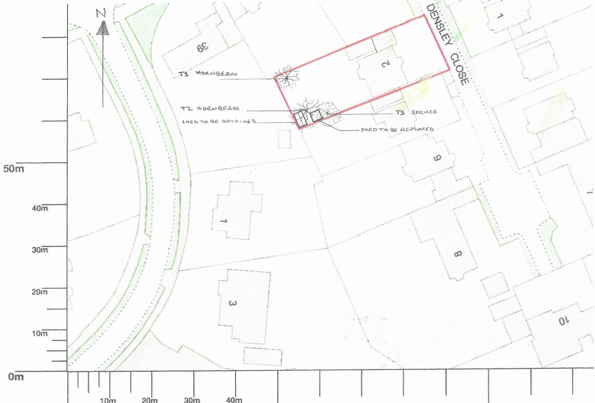
SCALE 1:500 AT A4 TREE PLAN 2 DENSLEY CLOSE, WGC, AL8 7JX
