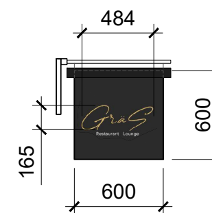
Externally lit hanging sign Font: Bespoke flat Colour: Background Black Text: White + Gold Lights: External white LED Lumen: 800lm Candela: ~ 400 cd
