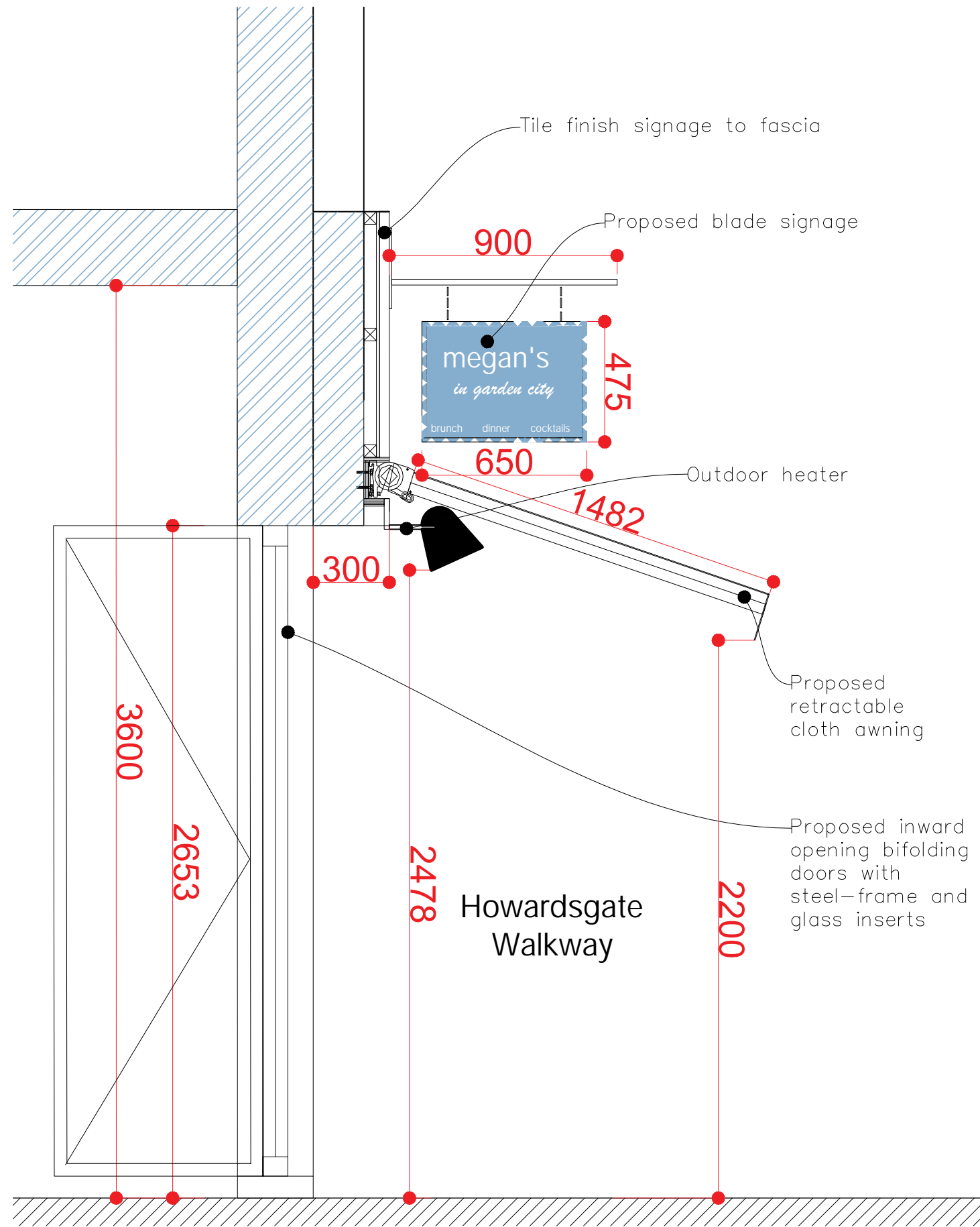
02 Proposed Shopfront Section 1:20 @ A3
