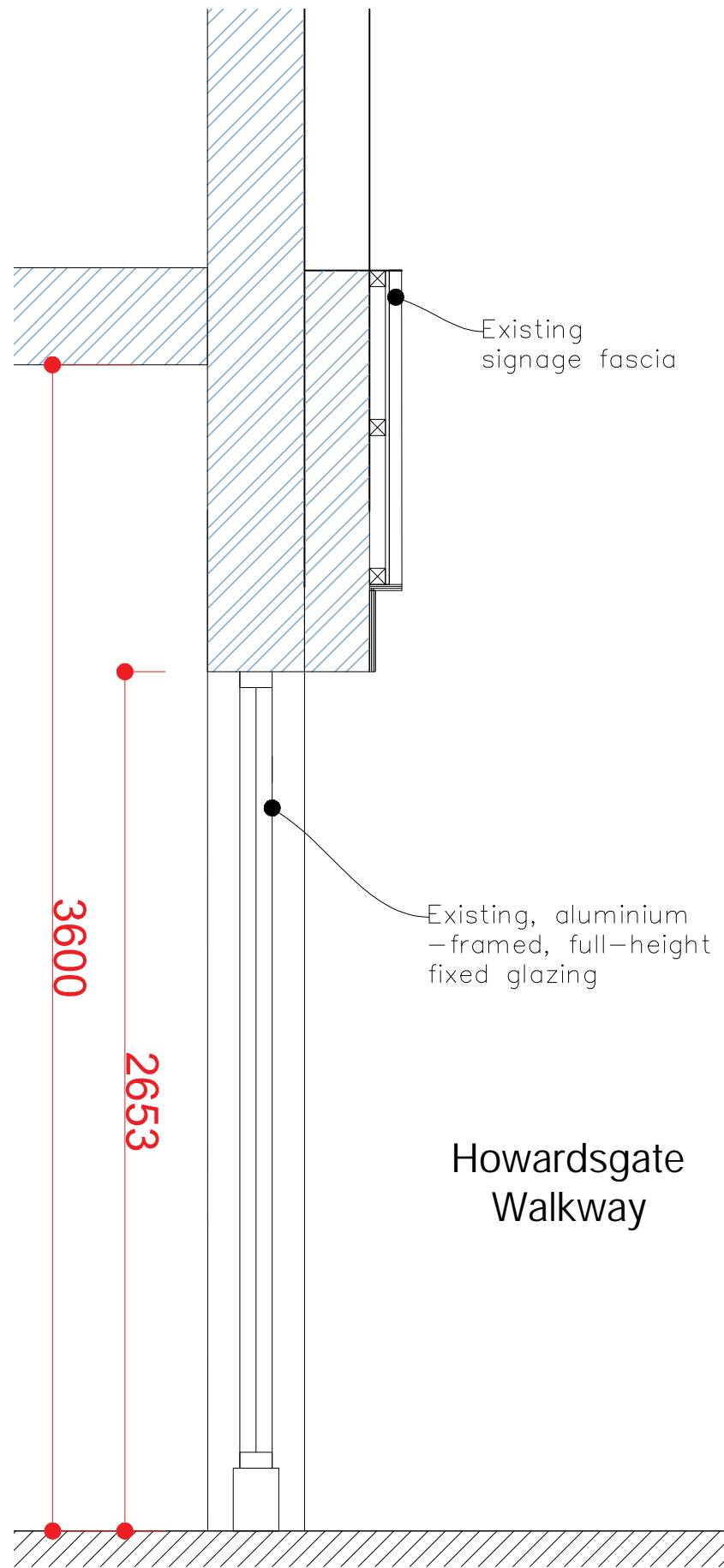
01 Existing Shopfront Section 1:20 @ A3
