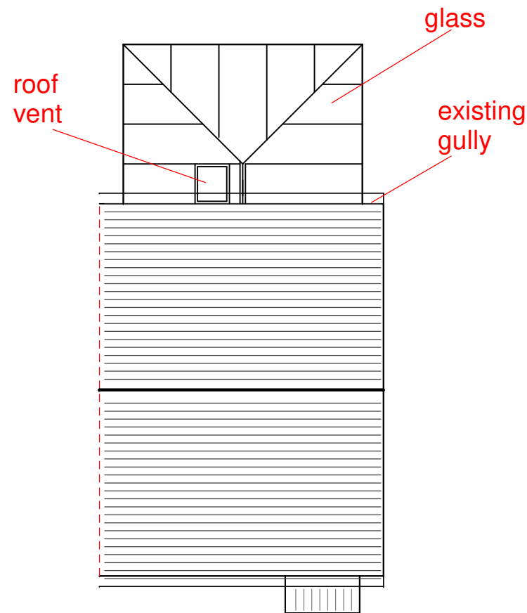
ROOF PLAN
