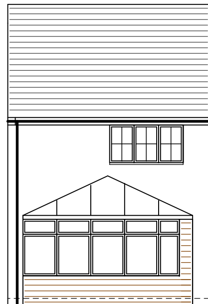
rear (south west) elevation
