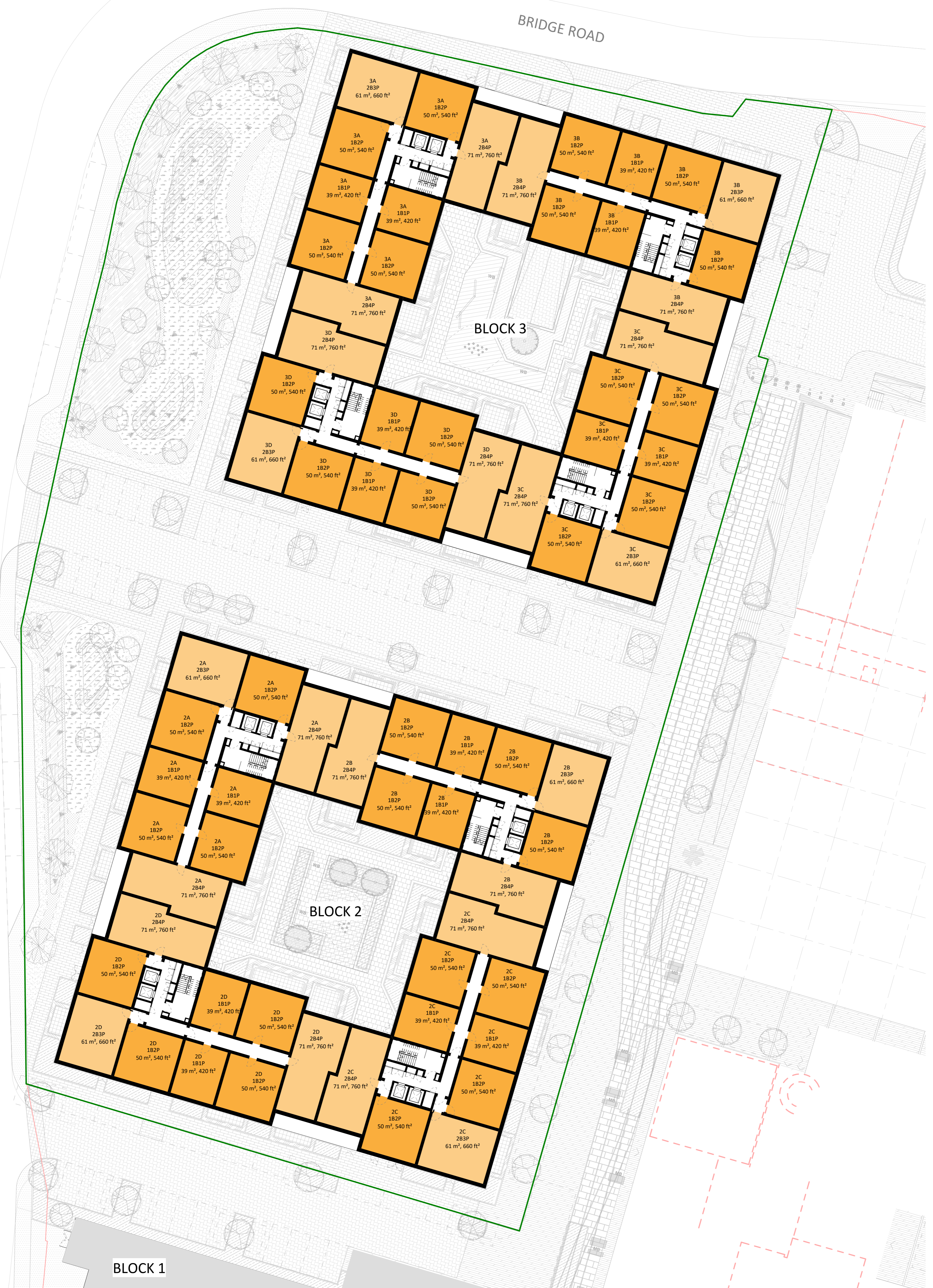
1 Indicative First Floor Plan - Blocks 2&3 1 : 250
