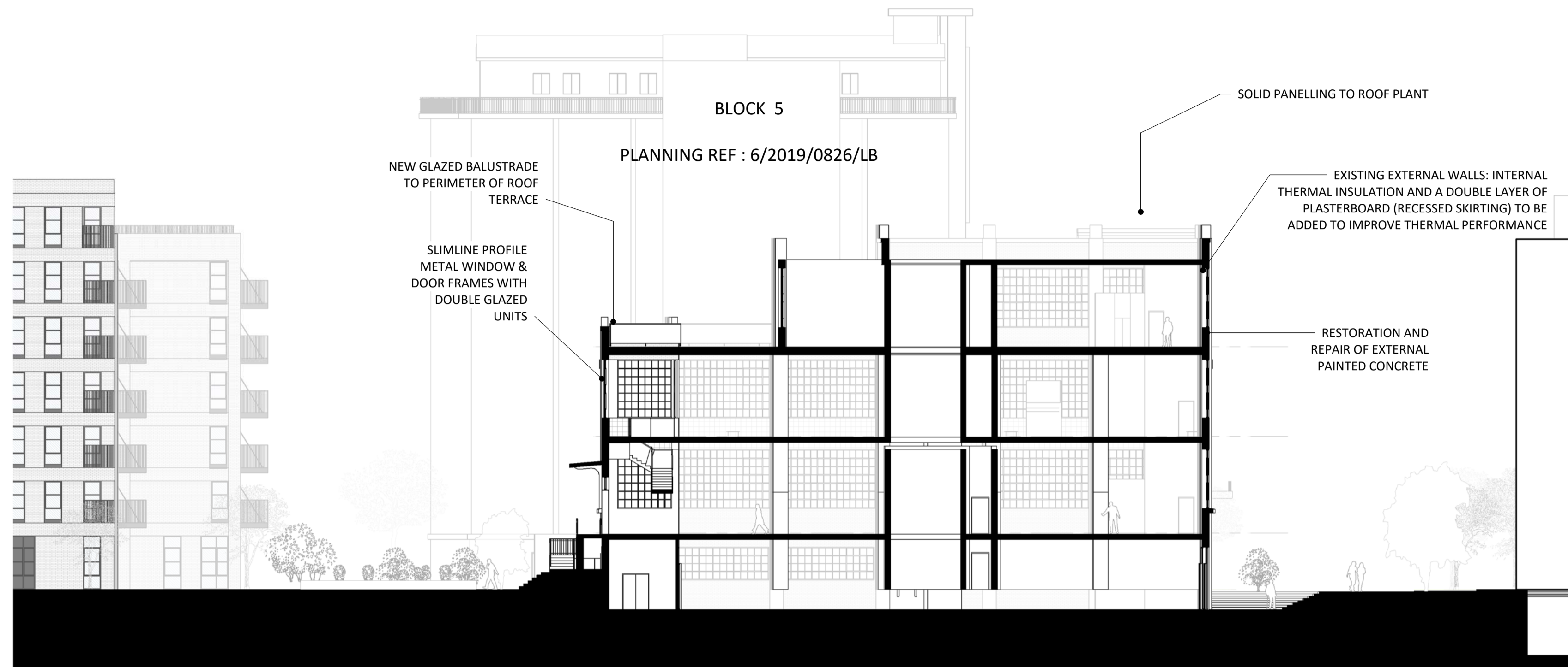
BLOCK 7 1 Section through Production Hall 1 : 200 @A1
