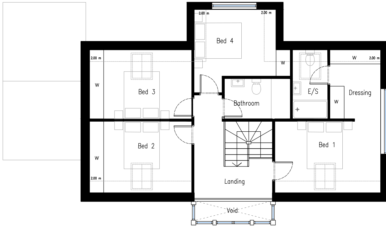
PROPOSED FIRST FLOOR PLAN, SETTLEMENT UNIT 2 1:100
