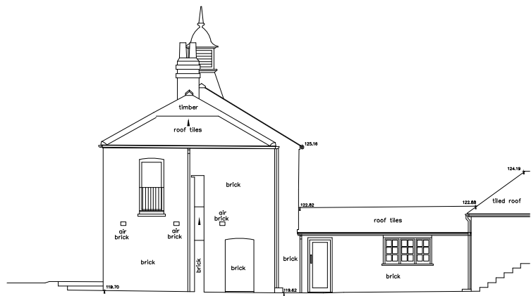
EXISTING BALLROOM WING SOUTH ELEVATION 1:200
