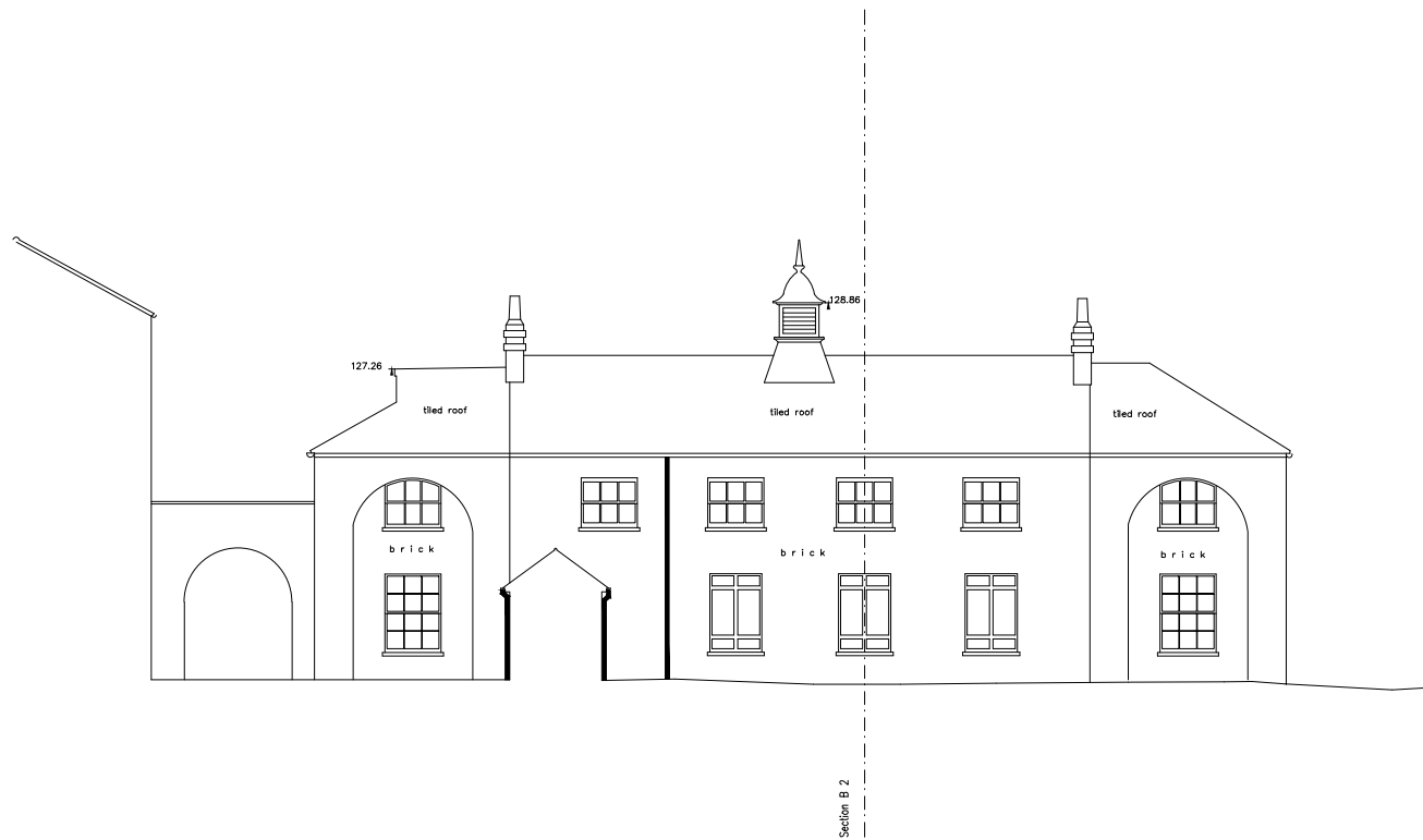
EXISTING BALLROOM WING EAST ELEVATION 1:200
