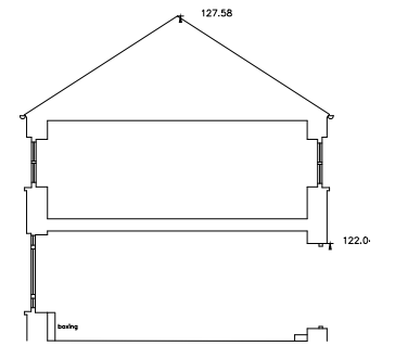
EXISTING BALLROOM SECTION B2 1:200
