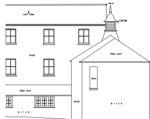
EXISTING BALLROOM NORTH ELEVATION 1:200
