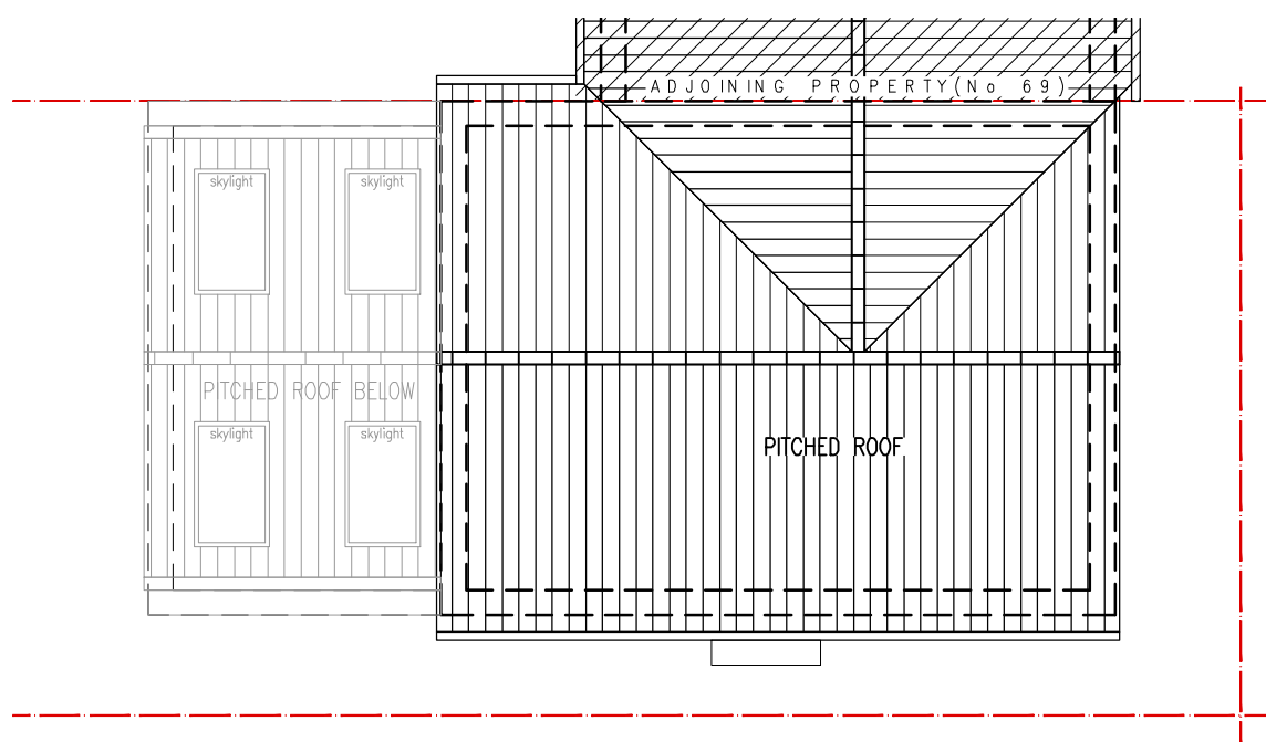
[03] PROPOSED ROOF PLAN
