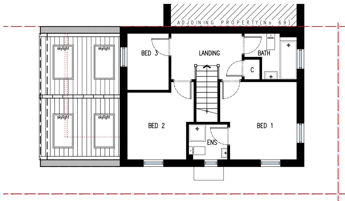
[02] PROPOSED FIRST FLOOR PLAN
