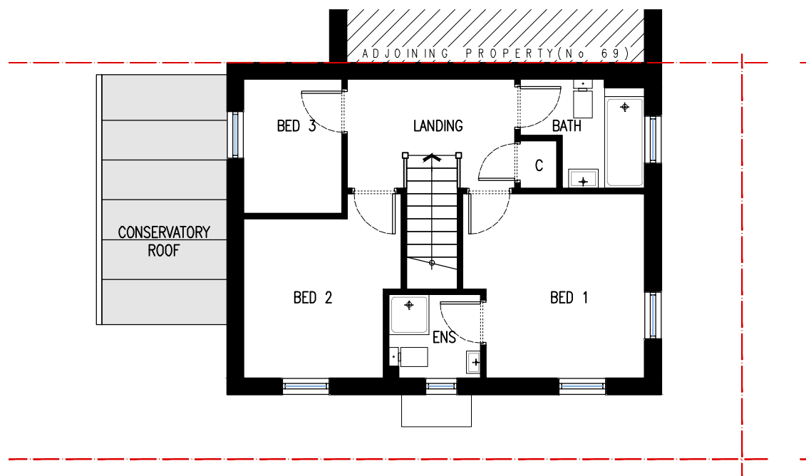
[02] EXISTING FIRST FLOOR PLAN
