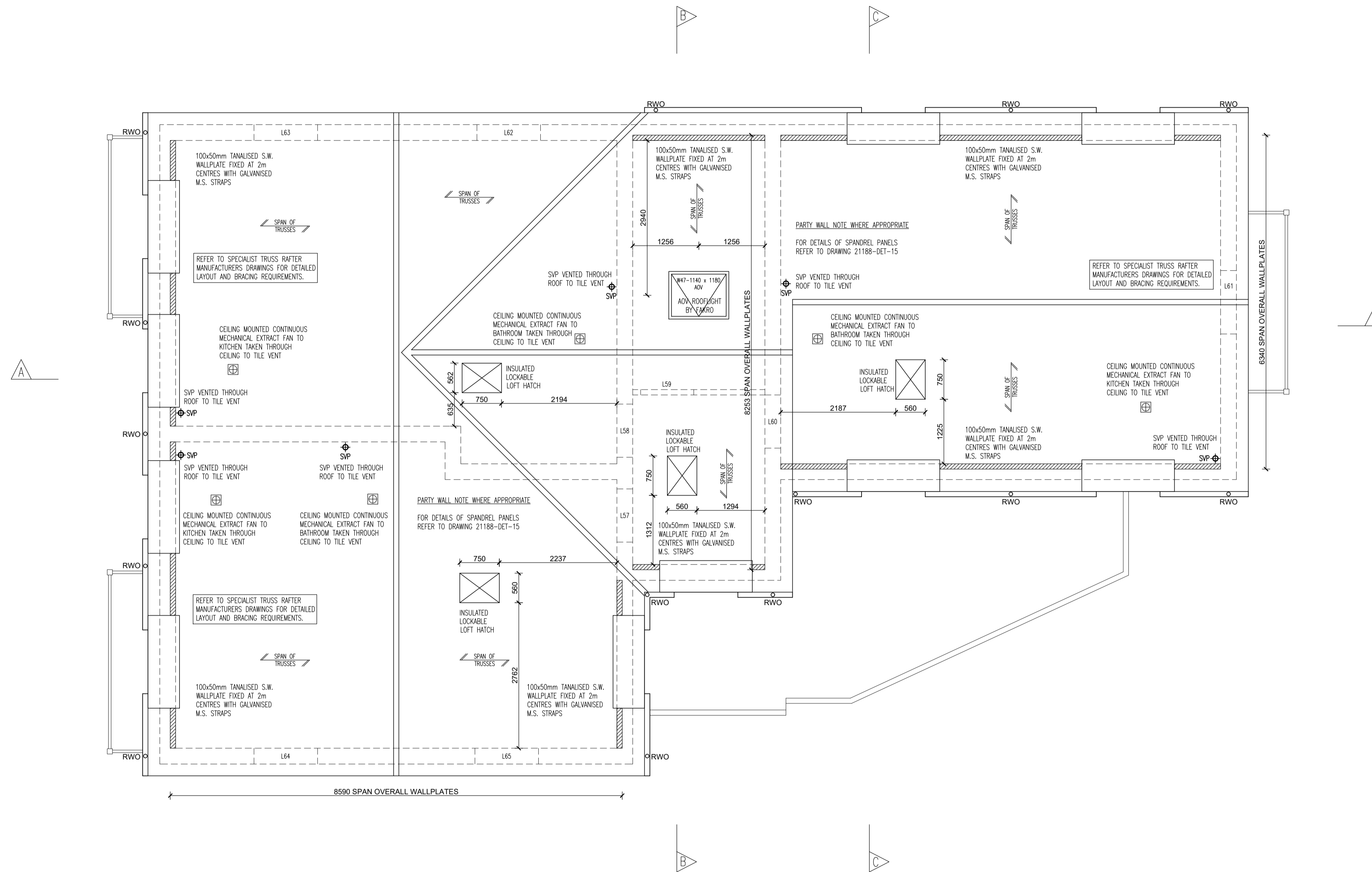
ROOF PLAN
