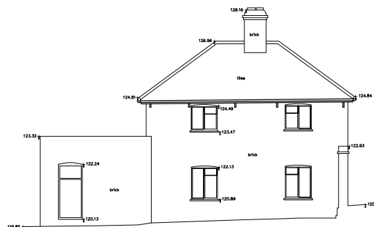
EXISTING WEST ELEVATION, OAK COTTAGE 1:200
