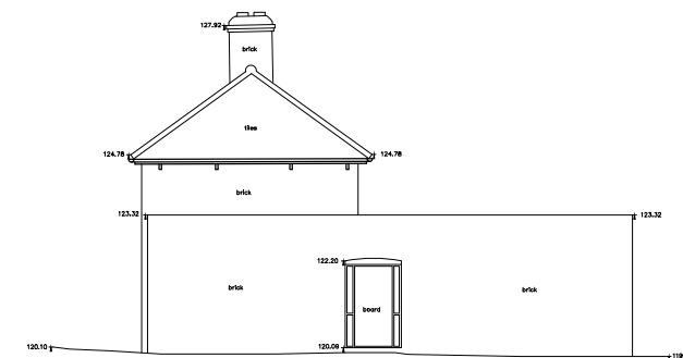
EXISTING NORTH ELEVATION, OAK COTTAGE 1:200
