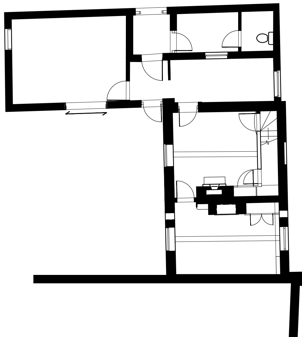
EXISTING GROUND FLOOR PLAN, OAK COTTAGE 1:100
