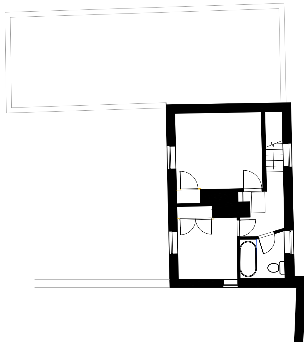
EXISTING FIRST FLOOR PLAN, OAK COTTAGE 1:100
