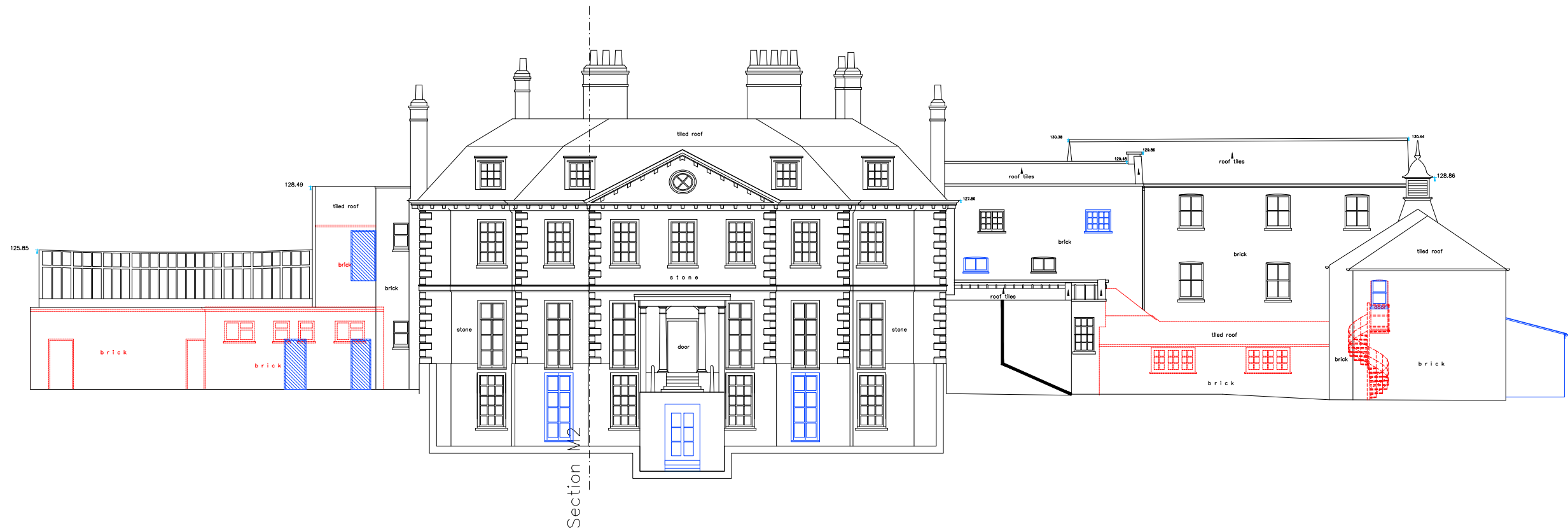
PROPOSED NORTH ELEVATION, NORTHAW HOUSE AND EDWARDIAN WING 1:200
