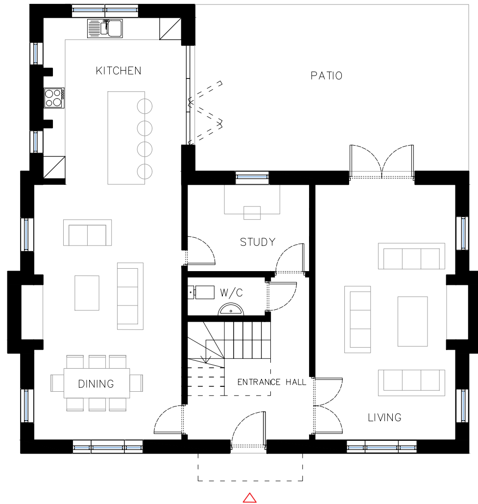
PROPOSED GROUND, FARM HOUSE 1:100
