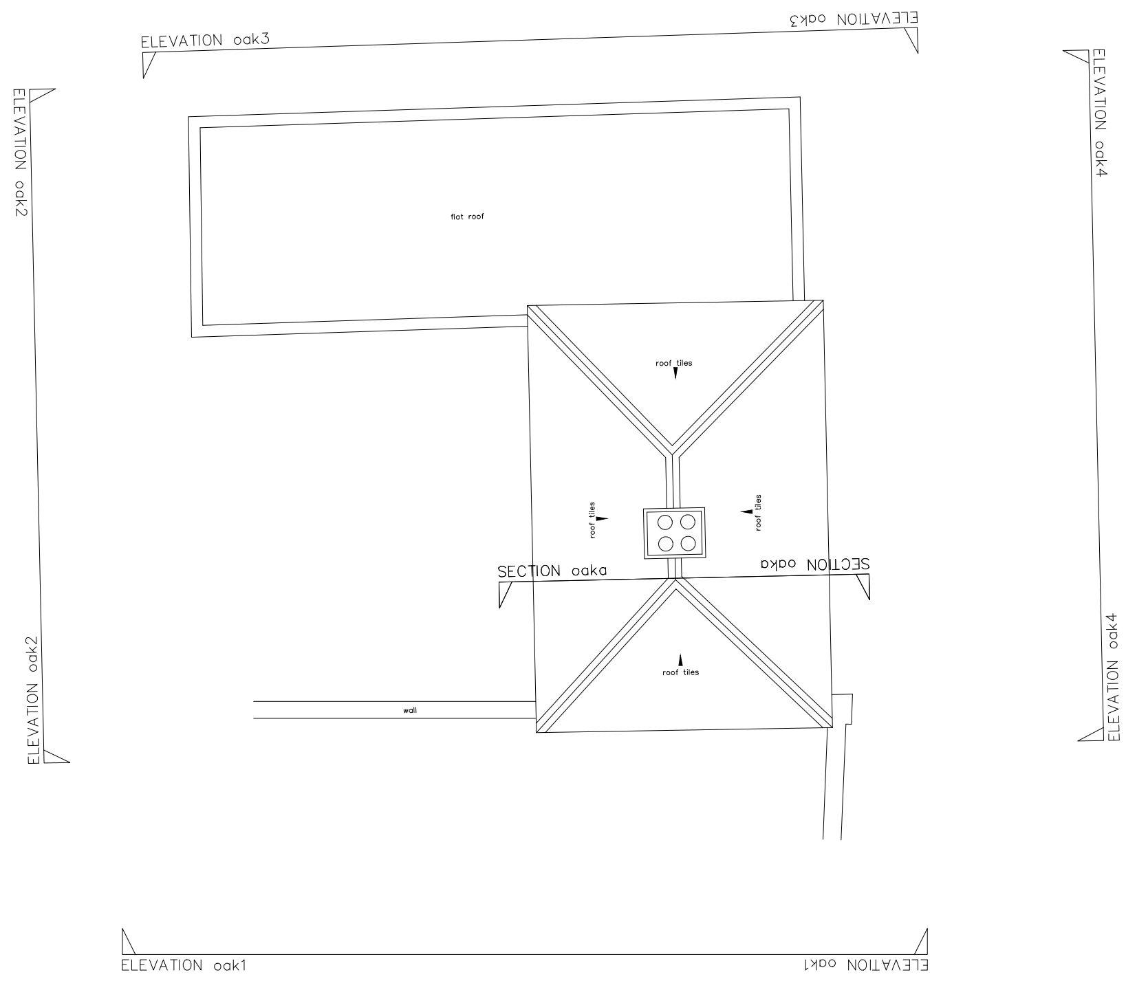
EXISTING ROOF PLAN, OAK COTTAGE 1:200
