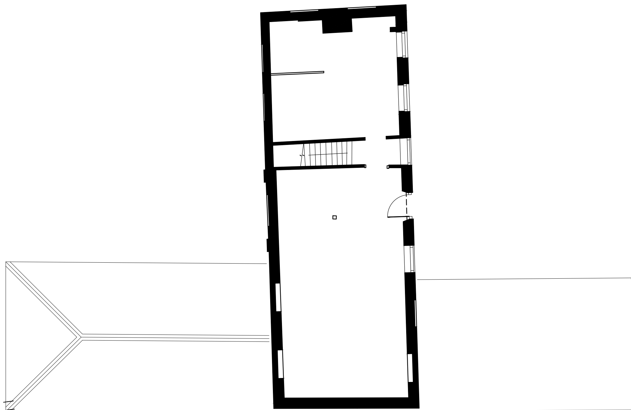
EXISTING FIRST FLOOR PLAN, STABLE BLOCK 1:100
