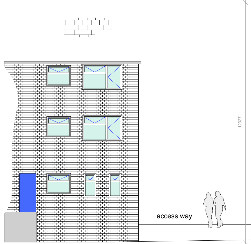
east elevation | rear view
