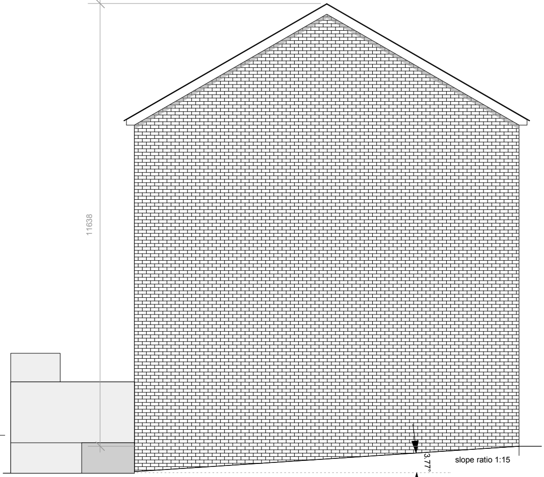
north elevation | side view from access way
