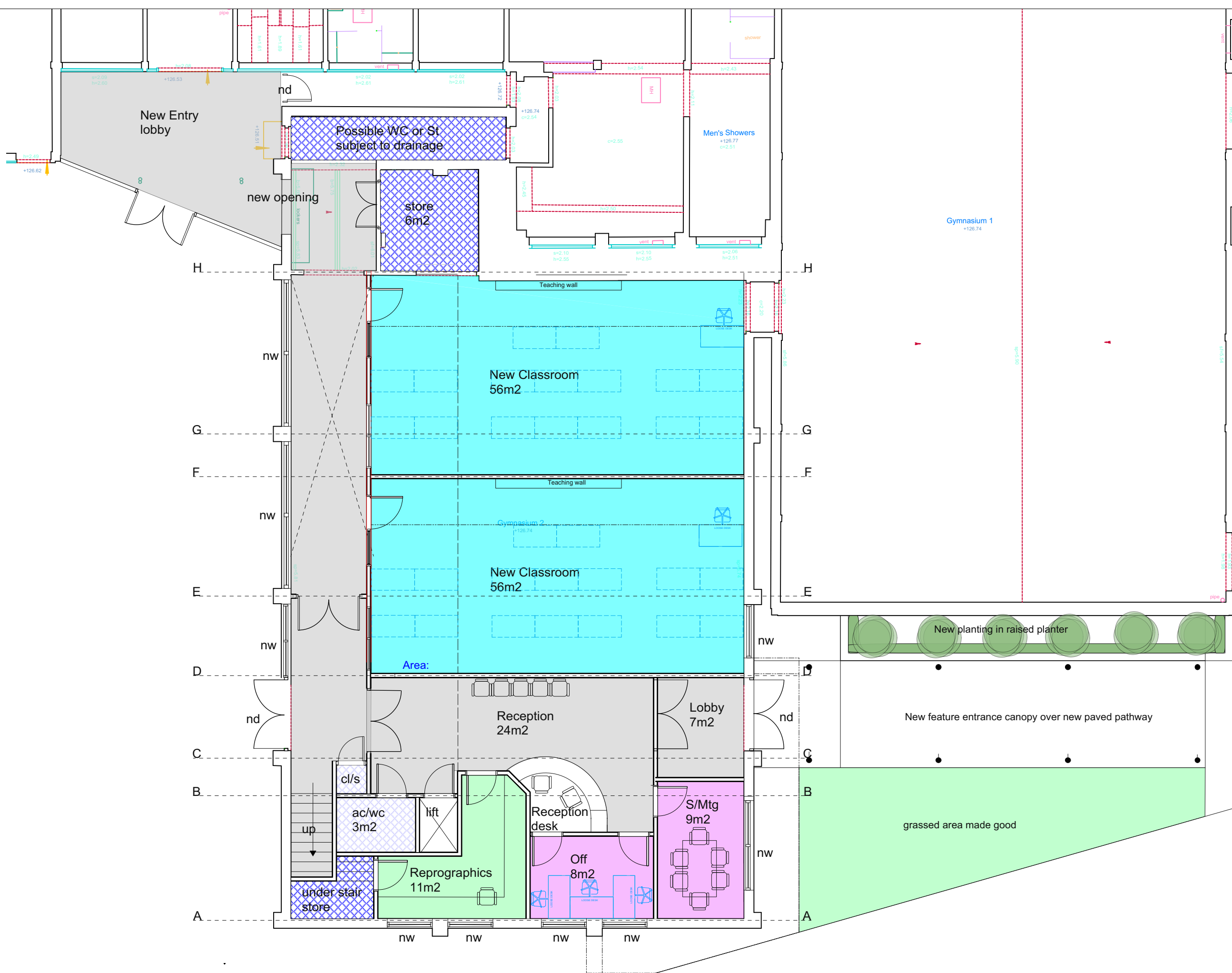
PROPOSED GROUND FLOOR PLAN 1:100
