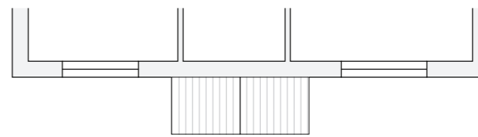
○ FIRST FLOOR PLAN, EXISTING SCALE 1:100
