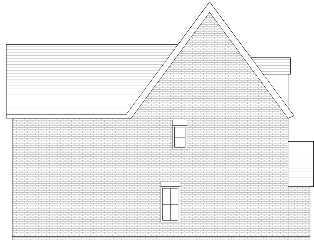
○ SIDE ELEVATION 1, PROPOSED SCALE 1:100
