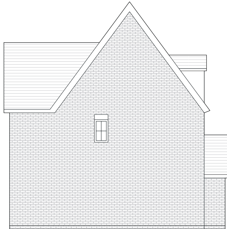
○ SIDE ELEVATION 1, EXISTING SCALE 1:100
