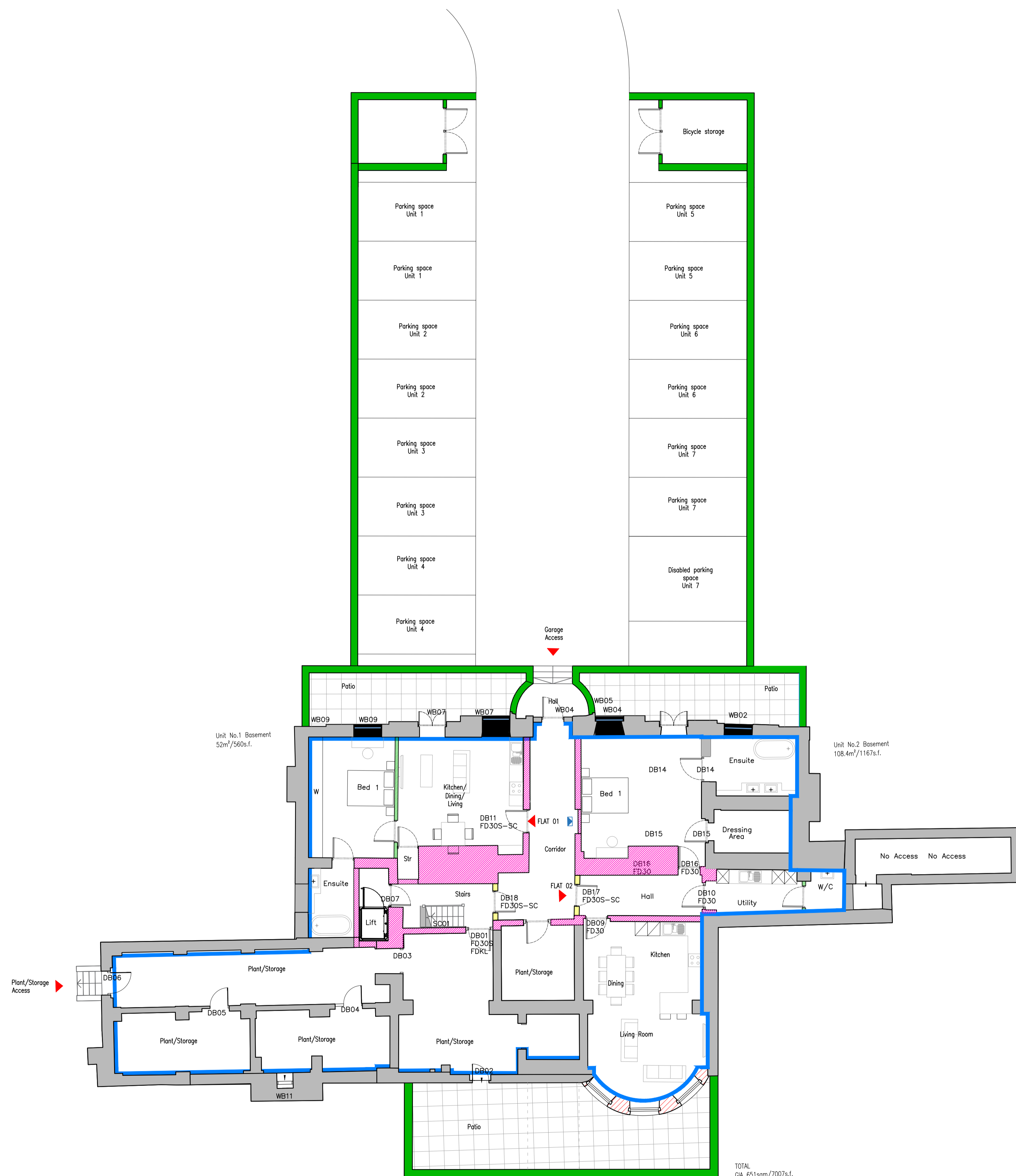
Basement Plan
