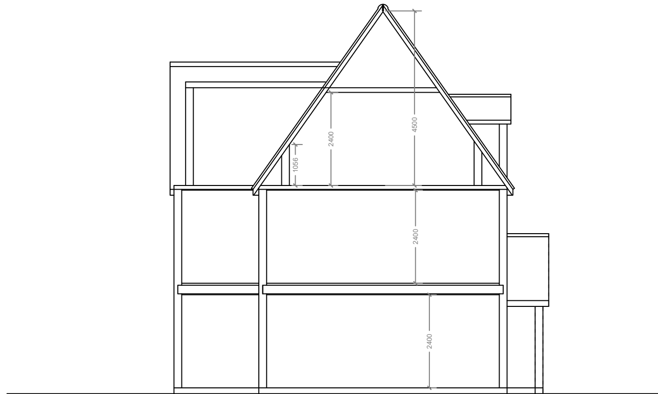
18 PROPOSED SECTION SCALE 1:100
