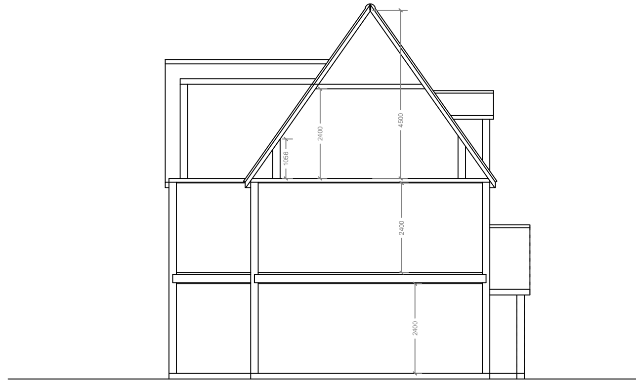
18 PROPOSED SECTION SCALE 1:100
