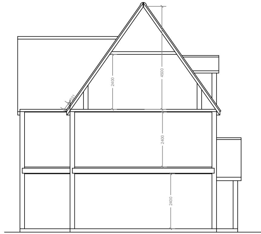
9 EXISTING SECTION SCALE 1:100
