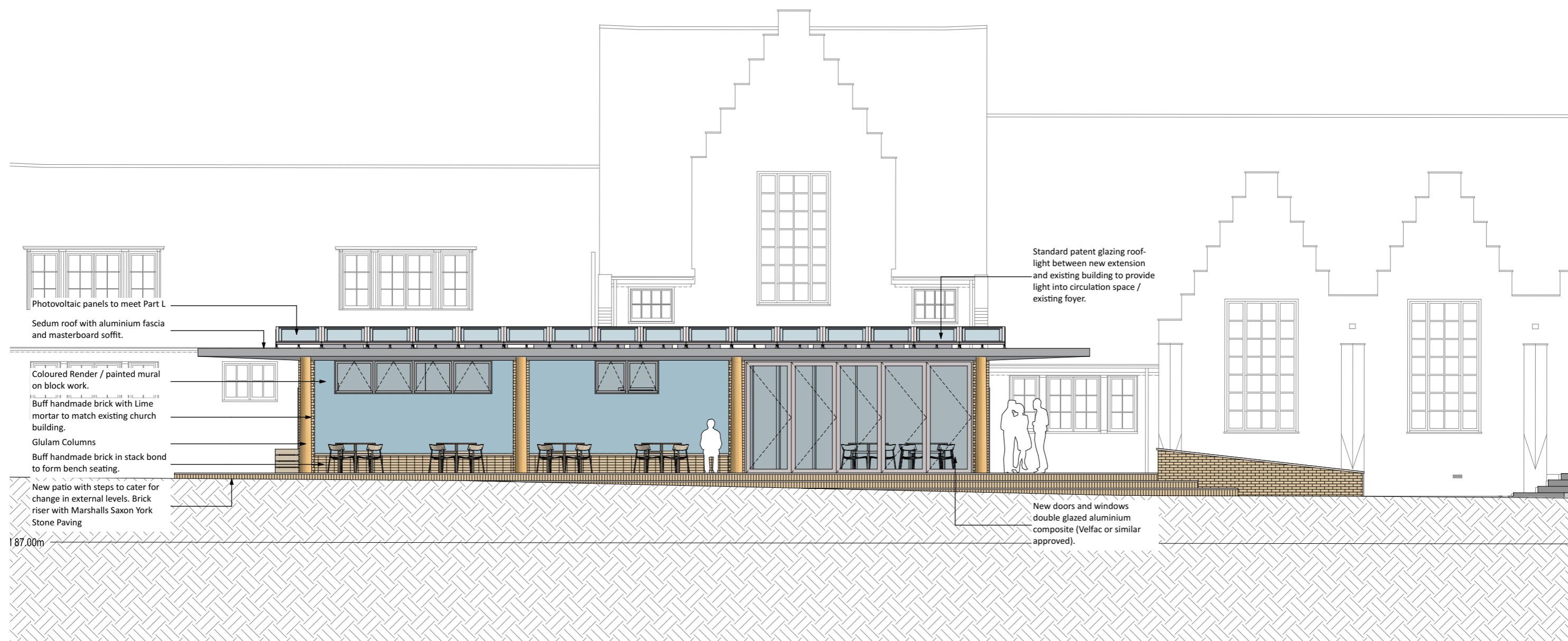
PROPOSED ELEVATION | South SCALE 1:100@A3
