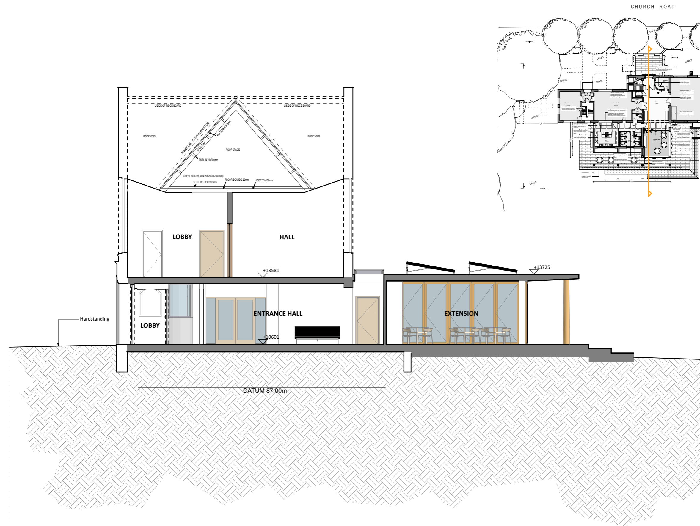
SECTION AA | Proposed SCALE 1:100@A3
