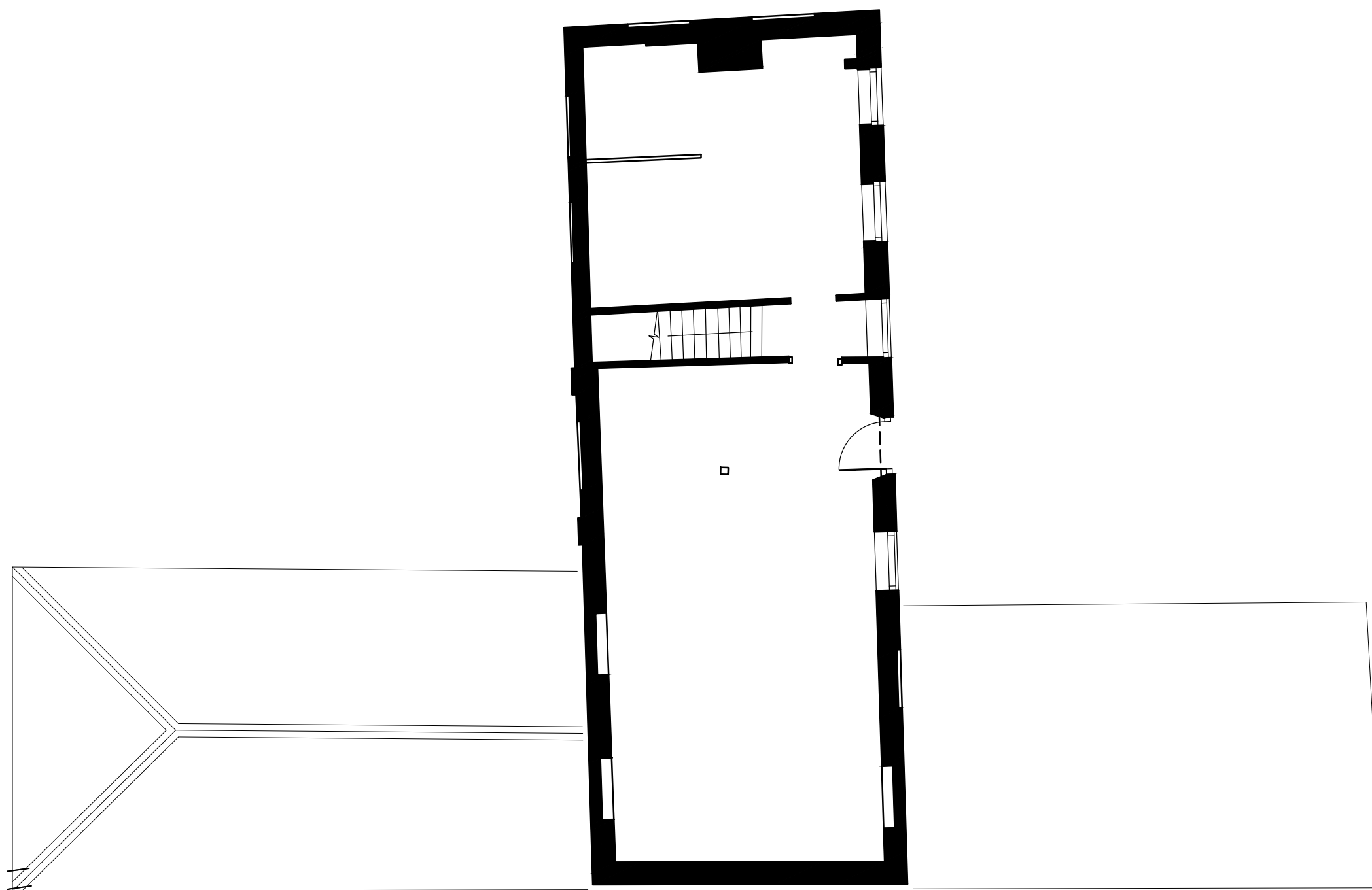
EXISTING FIRST FLOOR PLAN, STABLE BLOCK
