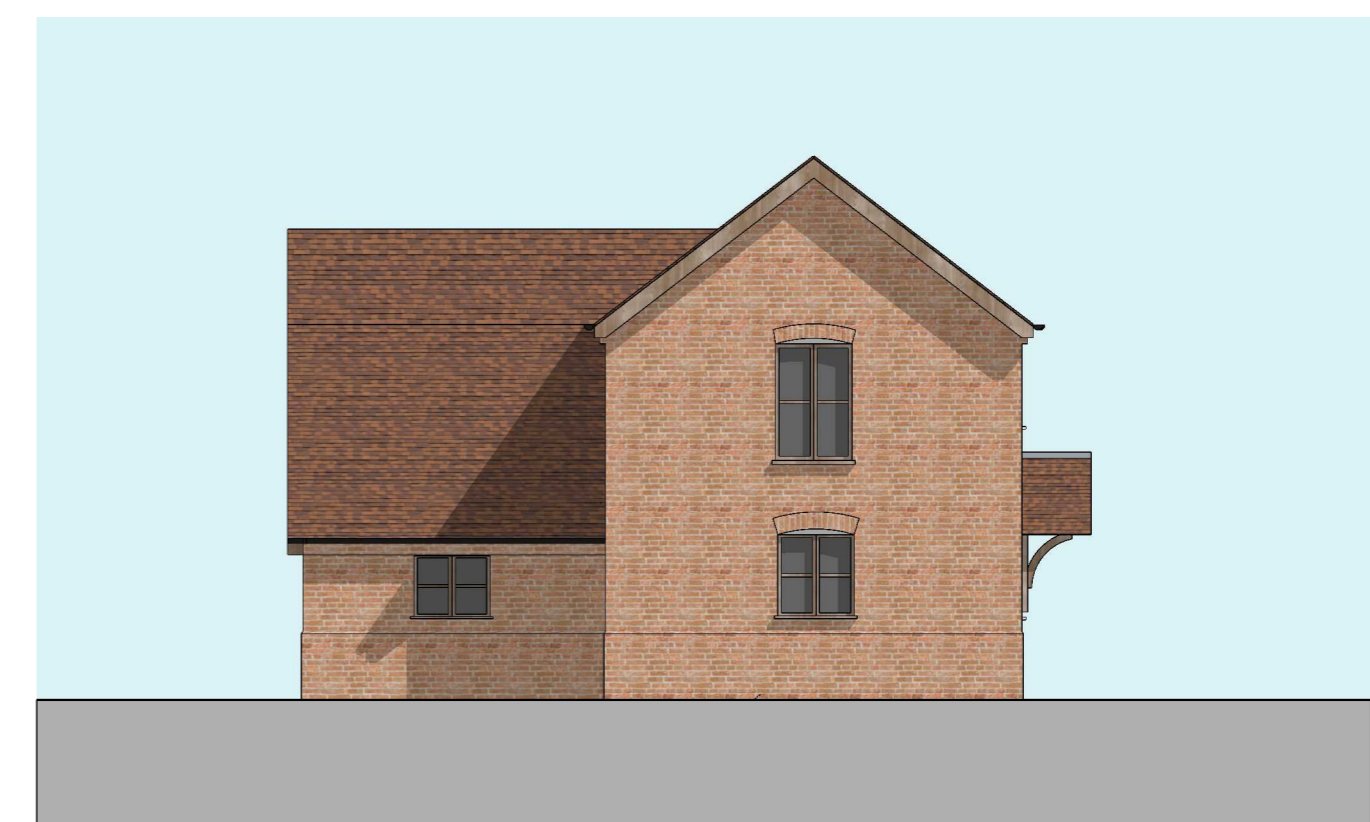
PROPOSED NORTH ELEVATION, DAIRY
