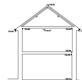
EXISTING SECTION, OAK COTTAGE 1:200
