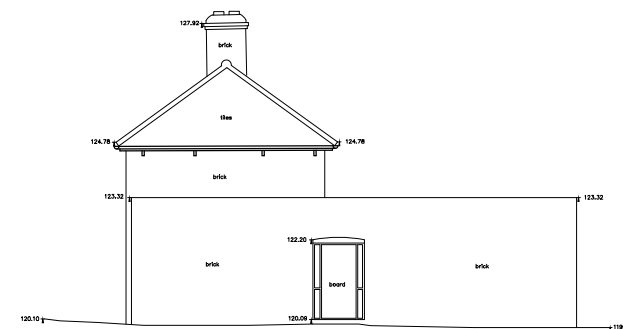
EXISTING NORTH ELEVATION, OAK COTTAGE 1:200
