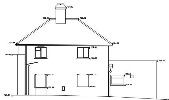
EXISTING EAST ELEVATION, OAK COTTAGE 1:200
