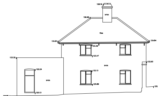
EXISTING WEST ELEVATION, OAK COTTAGE 1:200
