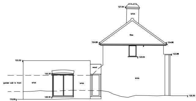
EXISTING SOUTH ELEVATION, OAK COTTAGE 1:200
