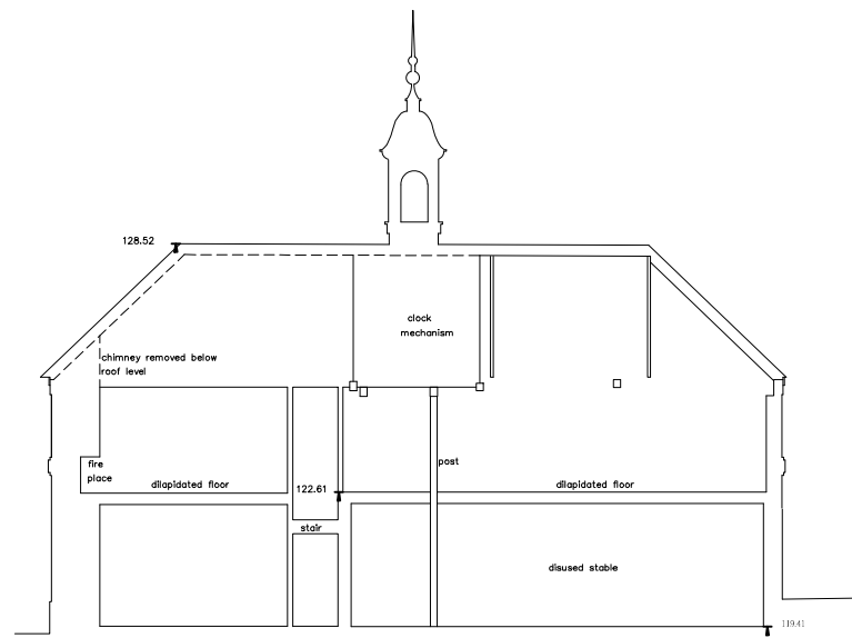
EXISTING SECTION S 1, STABLE BLOCK 1:200
