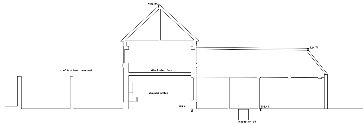
EXISTING SECTION S 2, STABLE BLOCK 1:200
