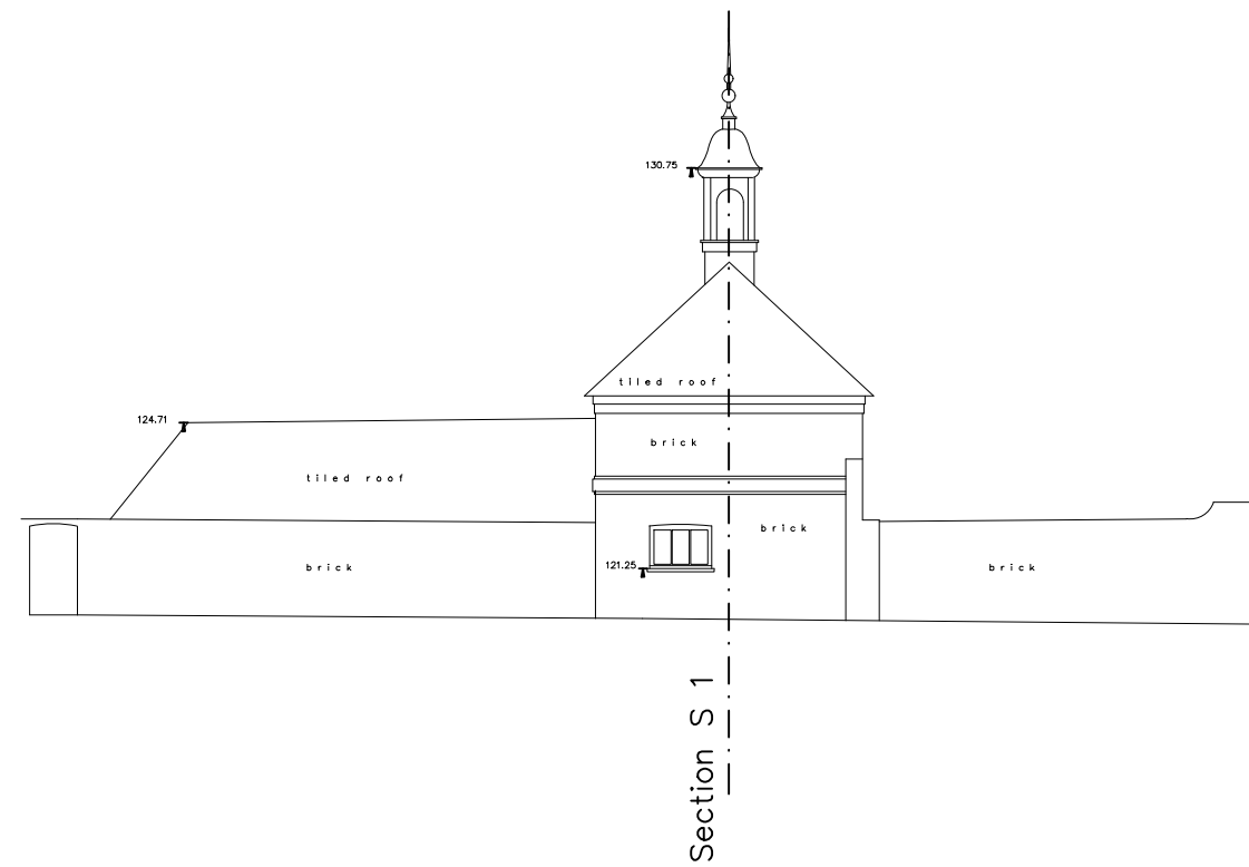
EXISTING SOUTH ELEVATION, STABLE BLOCK 1:200
