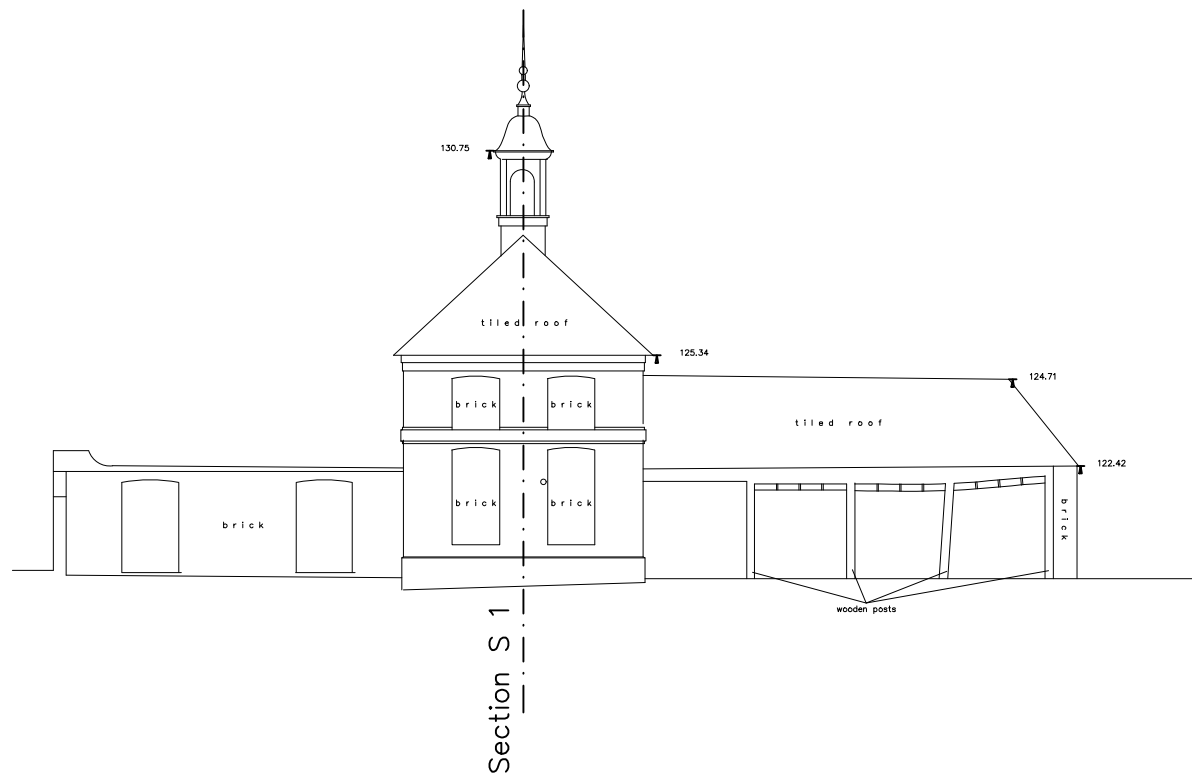
EXISTING NORTH ELEVATION, STABLE BLOCK 1:200
