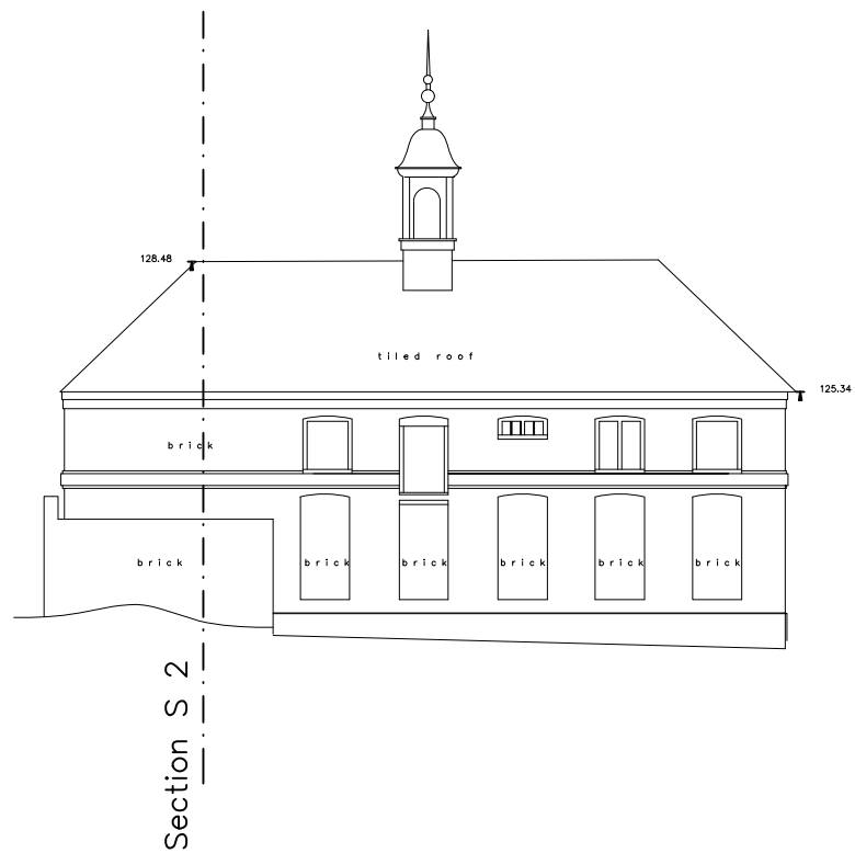
EXISTING EAST ELEVATION, STABLE BLOCK 1:200
