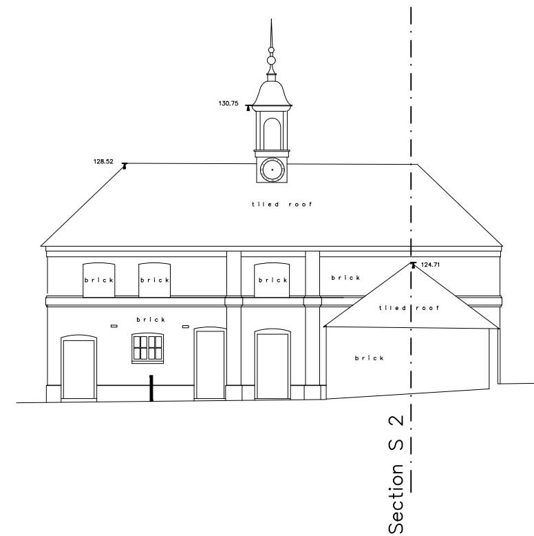
EXISTING WEST ELEVATION, STABLE BLOCK 1:200
