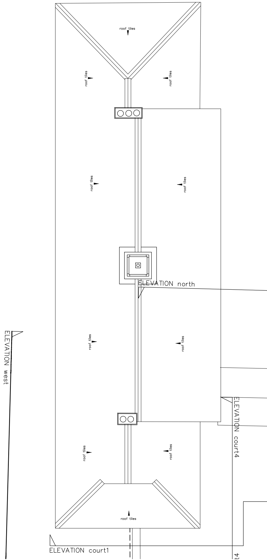
EXISTING ROOF PLAN, BALLROOM WING 1:100
