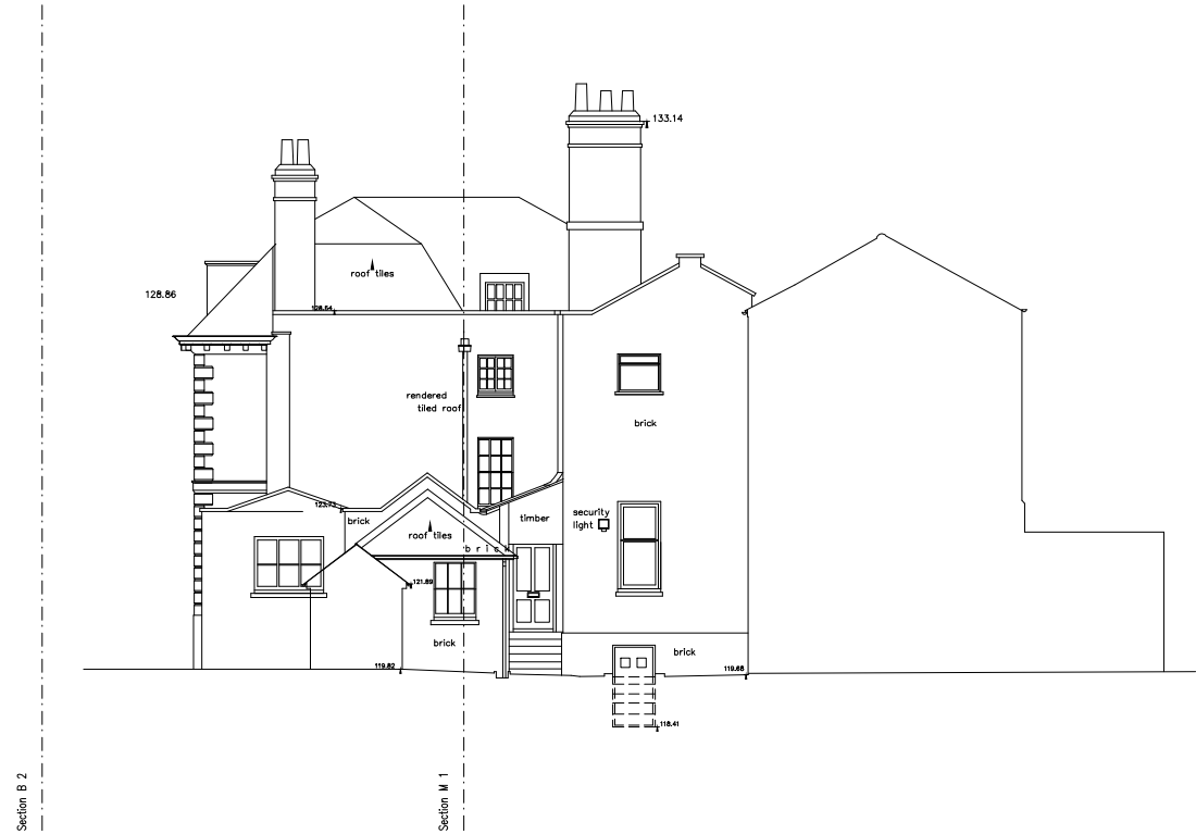
EXISTING WEST RETURN ELEVATION (A), NORTHAW HOUSE 1:200
