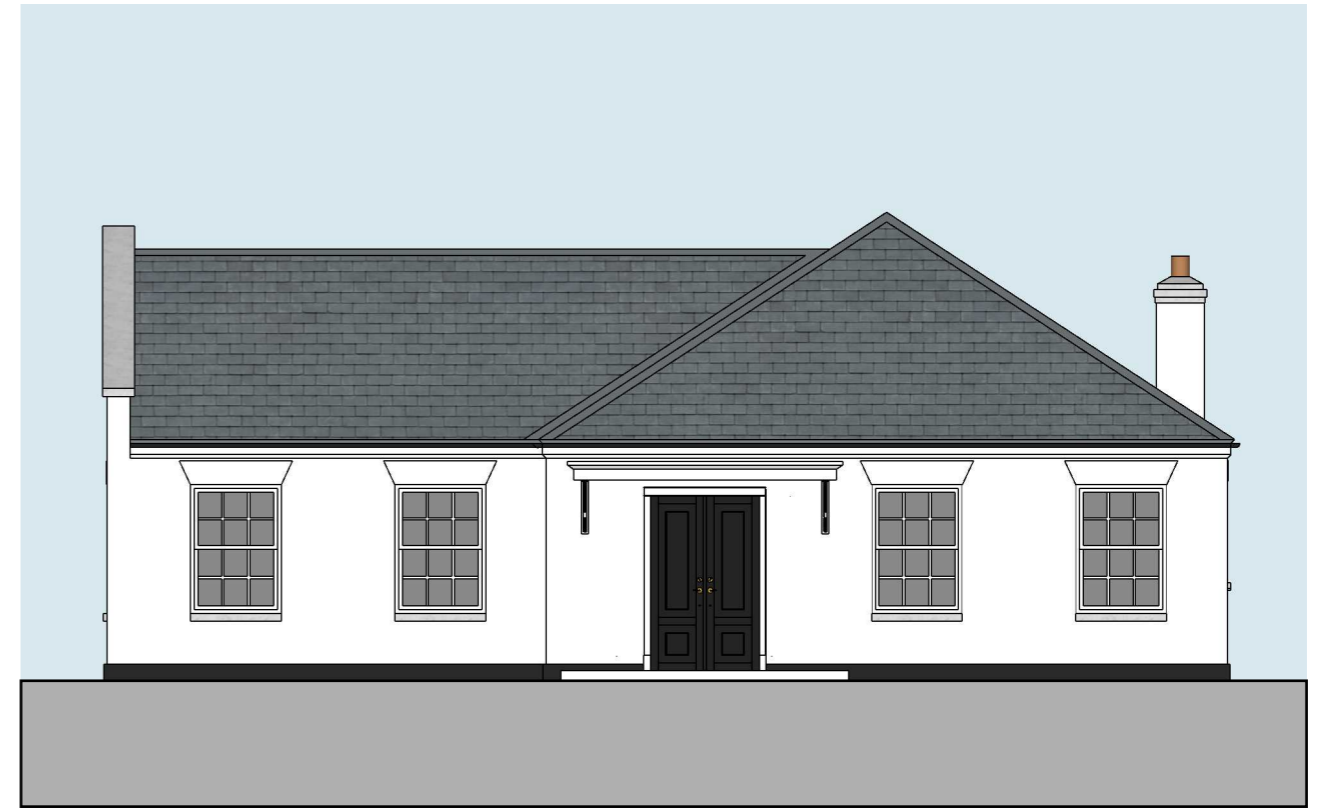
NORTH ELEVATION
