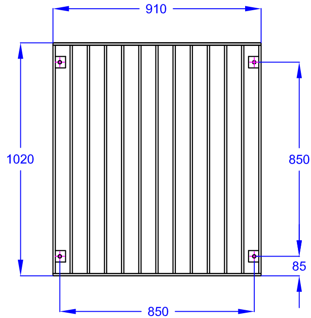
H10C Headwall grating
