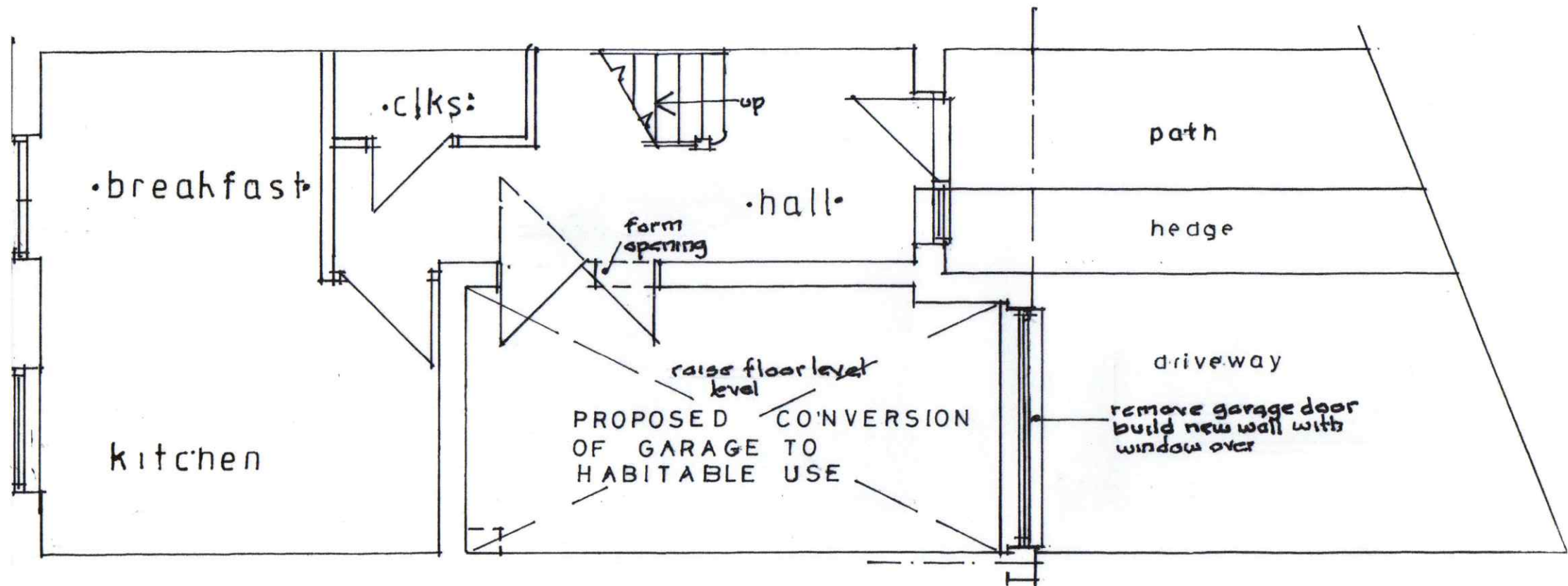
•ground floor plan. •scale. 1:50.
