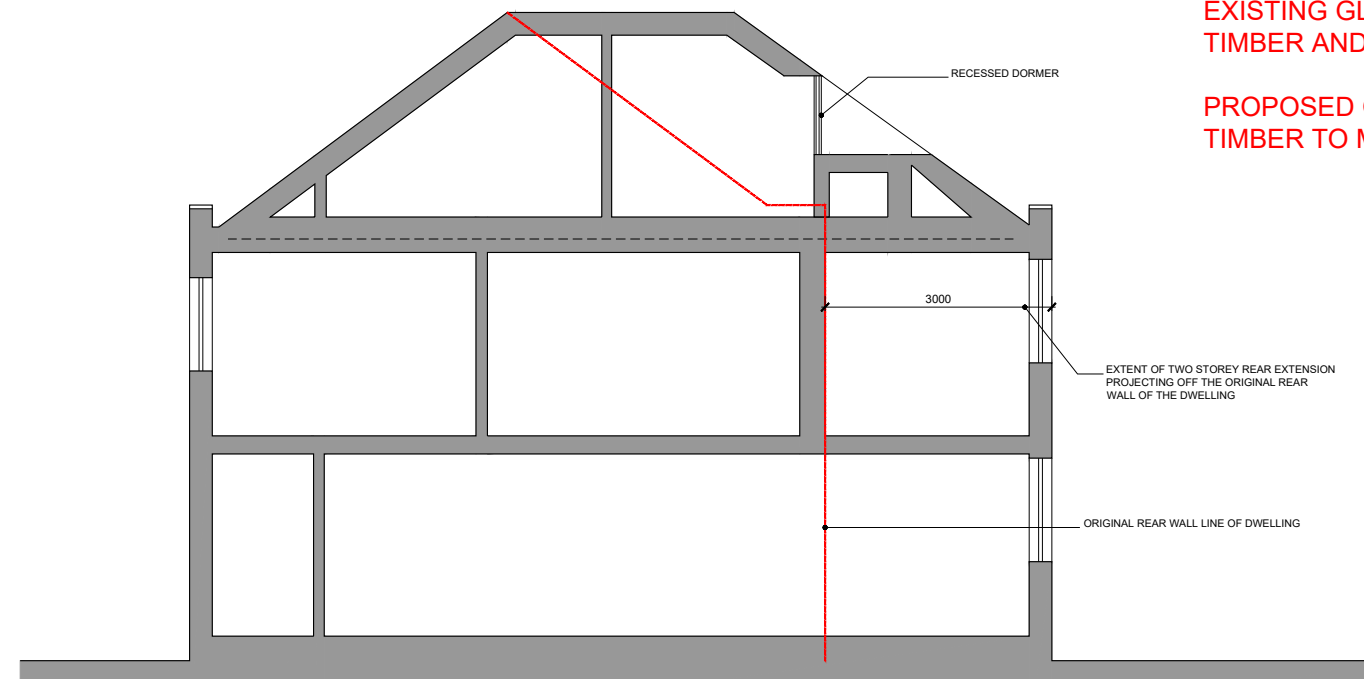
2 PROPOSED SIDE SECTION SK-008 SCALE@A1 1:50 SCALE@A3 1:100
