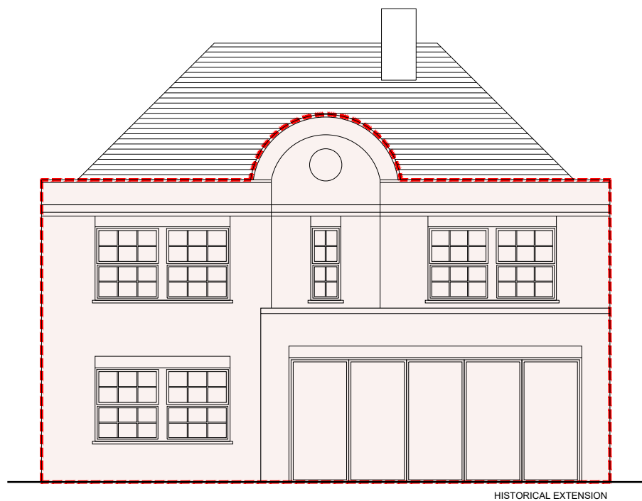
3 EXISTING REAR ELEVATION SK-004 SCALE@A1 1:50 SCALE@A3 1:100
