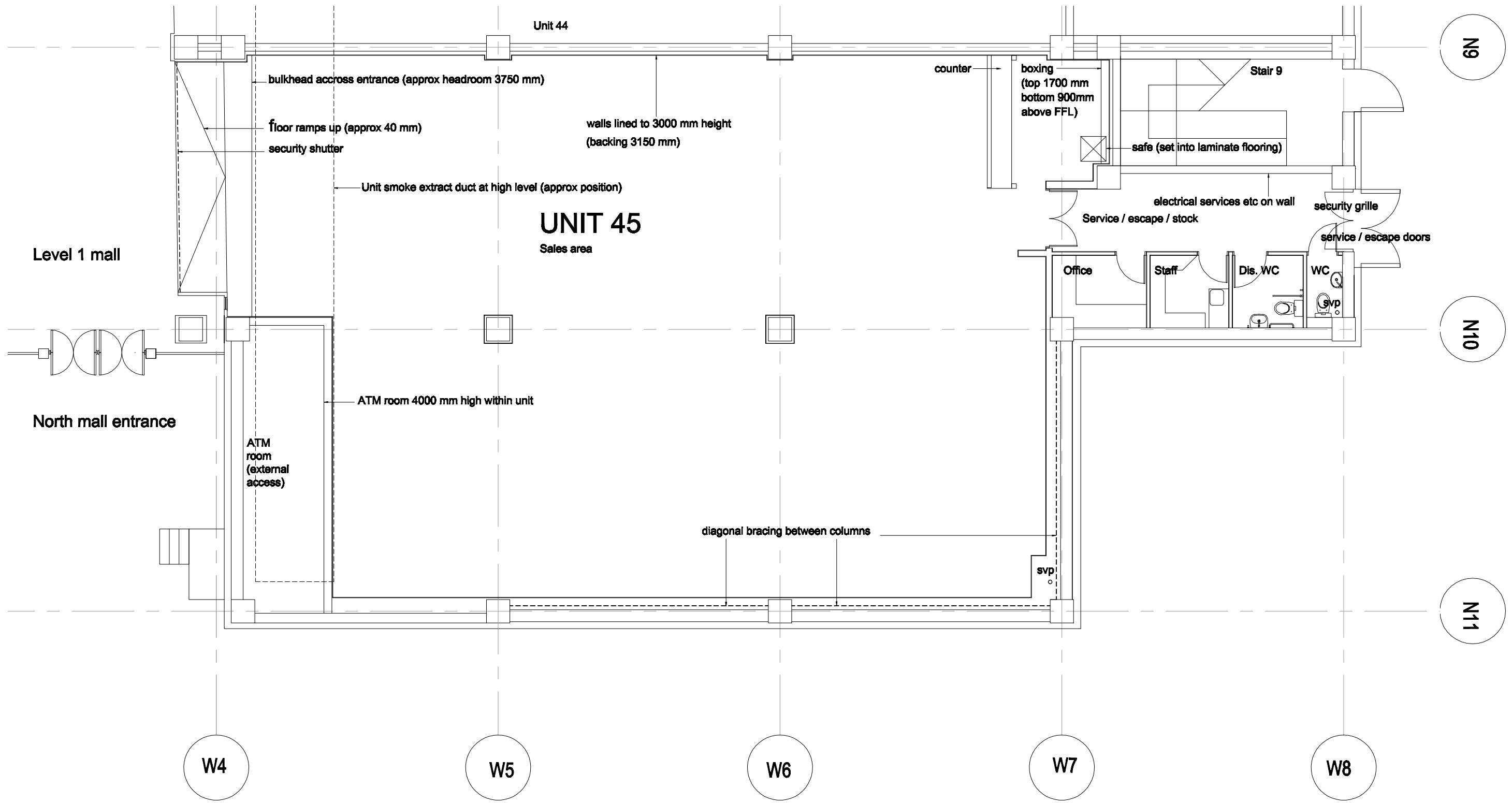
Unit 45 Plan (as existing) scale: 1:100@A3 13 June 2009 1578 SK01 P01
