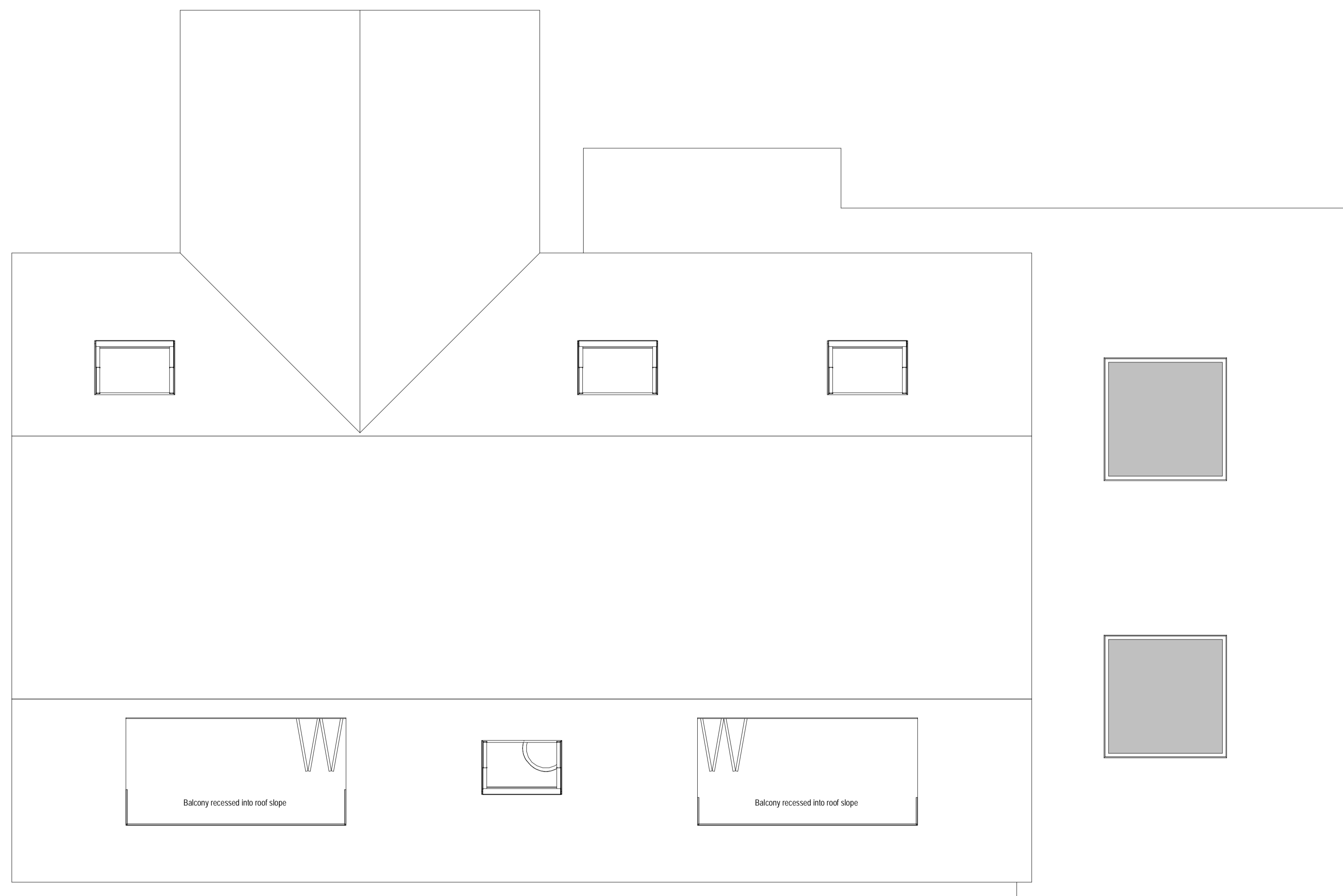
1 Proposed Roof Plan 1 : 50
