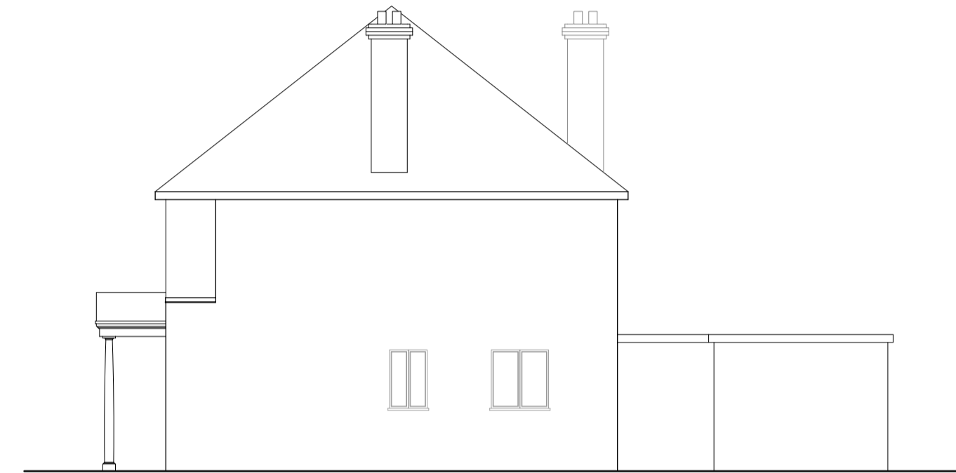
Existing (other) Side Elevation
