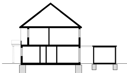
Existing Section AA
