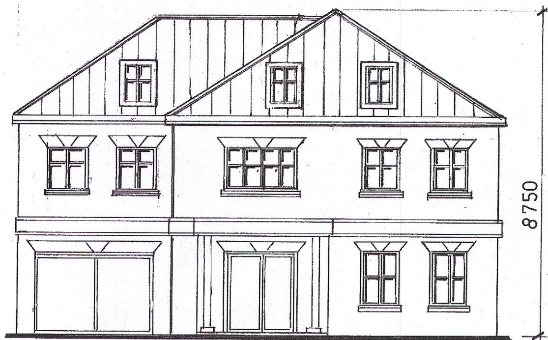
Proposed Front Elevation 1:100
